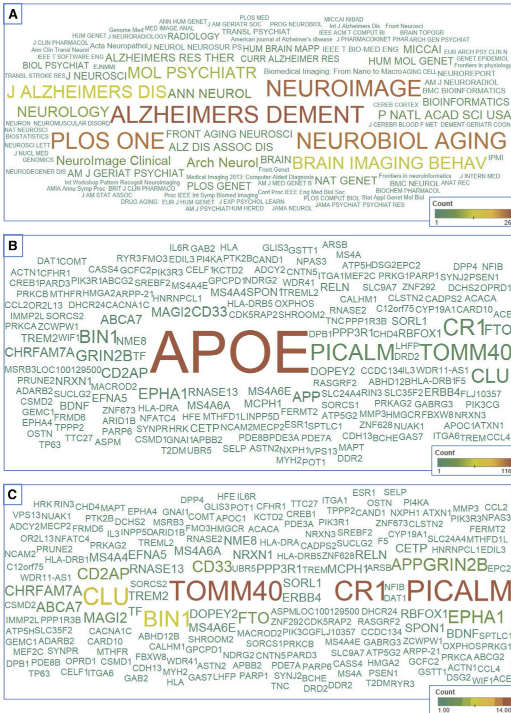
Fig. 2. Common journals and reported genes in manuscripts using ADNI genetic data. (A) A word cloud of journal names where articles using ADNI genetic data were published is shown with the color and size of a journal name corresponding to the number of articles published in that journal. Word clouds of gene names appearing in these article abstracts, (B) with and (C) without including APOE , are displayed with the color and size of a gene name corresponding to the number of abstracts mentioning the gene.
