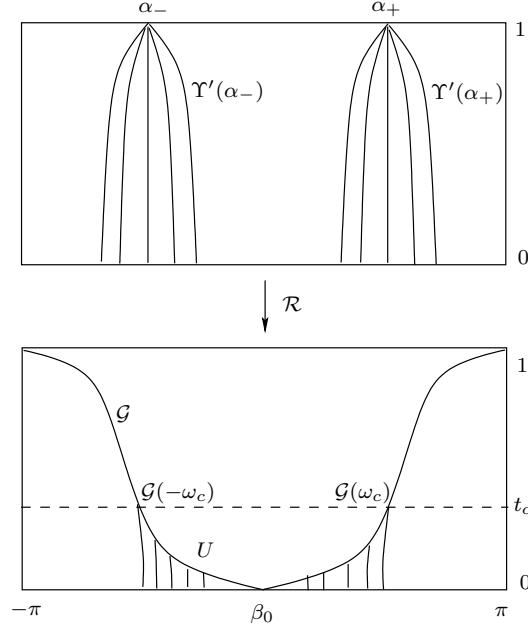
FIGURE 9.1. Topological triangles foliated by stable manifolds (below) and the corresponding stable tongues attached to the indeterminacy points \alpha_{\pm} (above).
