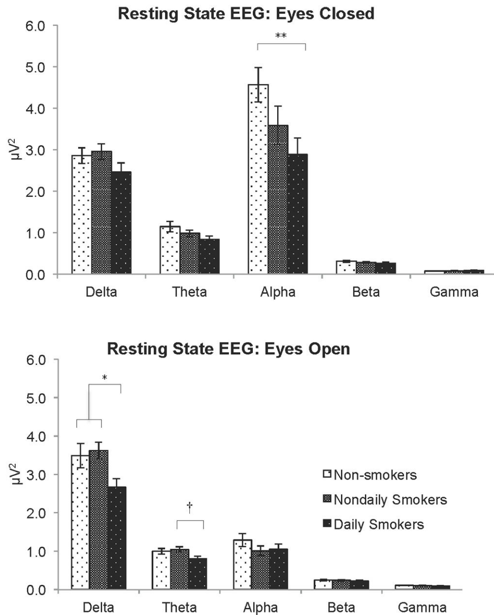
Figure 1. Resting State EEG power spectra for the eyes closed and eyes open conditions across groups. Delta: 1.5–3.5 Hz; Theta: 4–7.5 Hz; Alpha: 8–12.5 Hz; Beta (13–25 Hz; Gamma: 30–45 Hz. Error bars represent \pm 1 SEM. The following symbols represent significance: † p < .06 , * p < .05 , ** p < .01 .
