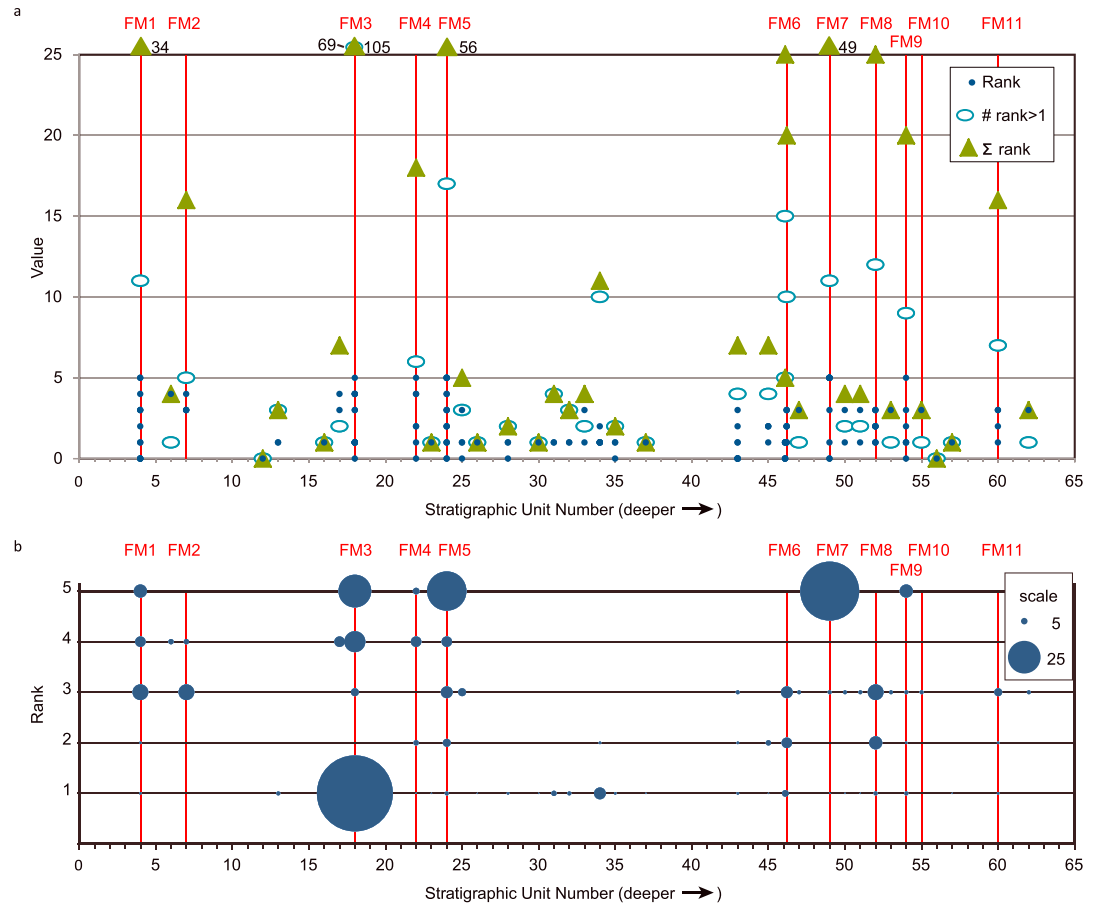
Figure 5. Combined plot of event indicator quality and number for all exposures of T1 based on ranking in Table 1 and catalogues in K. M. Scharer et al. [2014, 2015]. (a) Rank (1–5), the number of indicators with rank greater than 1, and the sum of the rank of indicators at all horizons. All of the qualified paleoearthquakes at Frazier Mountain (red lines) have at least one indicator with rank \geq 3 . Values greater than 25 are indicated at the top of the chart. (b) Alternate representation of the combined catalogue of event indicators to emphasize number of observations in each rank. The diameter of the symbol is scaled by the sum of the quality in each rank to illuminate the stratigraphic horizons with the largest number of high-quality indicators. For example, unit 4 has two indicators with a rank of 5, producing a symbol diameter of 10. Deformation at unit 18 (FM3) is unique as it includes a few high-quality indicators (5 indicators with rank 5) and many low-quality indicators (over 50 indicators with rank 1).
