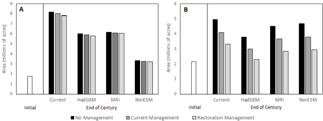
Figure 6. Projections of exotic grass (A) and juniper (phase I, II and III woodlands) (B) under four climate scenarios and three management scenarios. Results are summarized across the entire eastern Oregon study area. The left panel in each graph shows the initial mapped landscape conditions and the middle-right panels show projected average future conditions at the end of the century (2081–2100).
