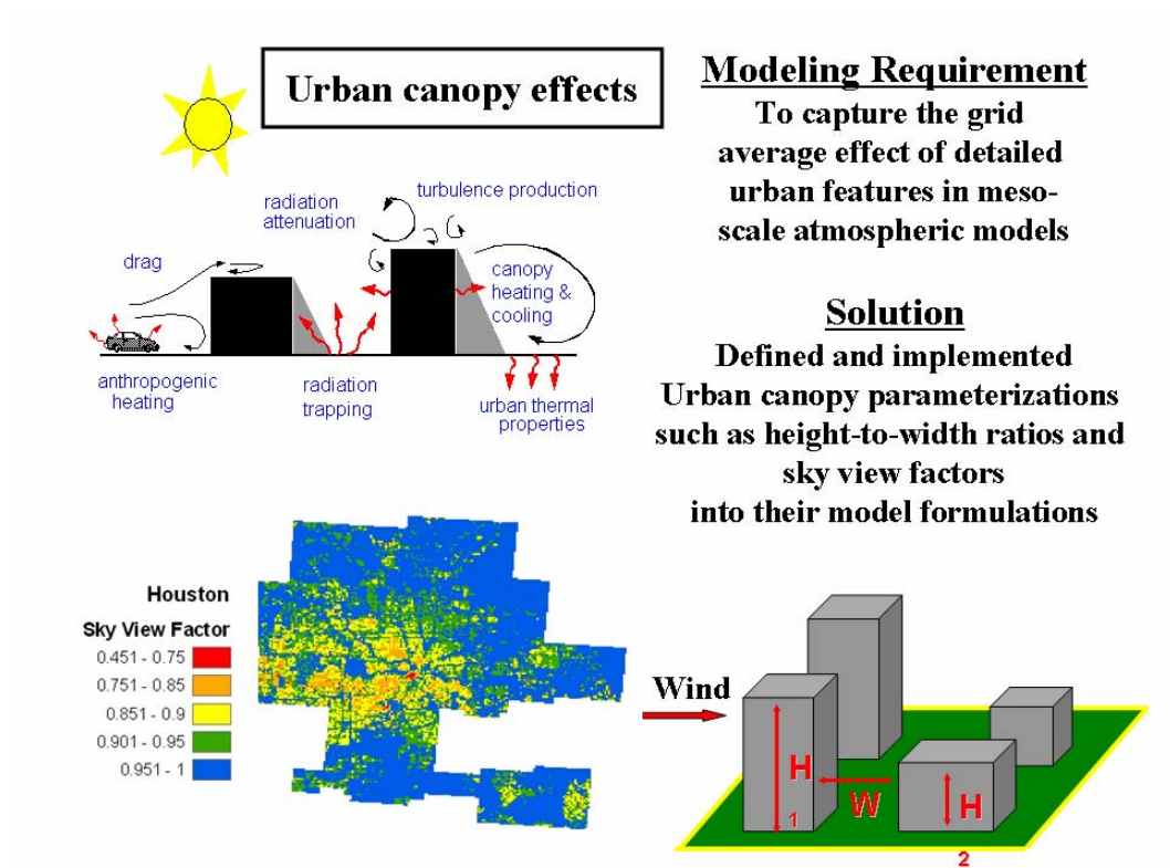
Figure 1: Schematic of urban canopy parameterization concept and methodology. Here, sky view factor is the ratio of the radiation received in the street canyon to the hemispheric radiation above the canopy.
