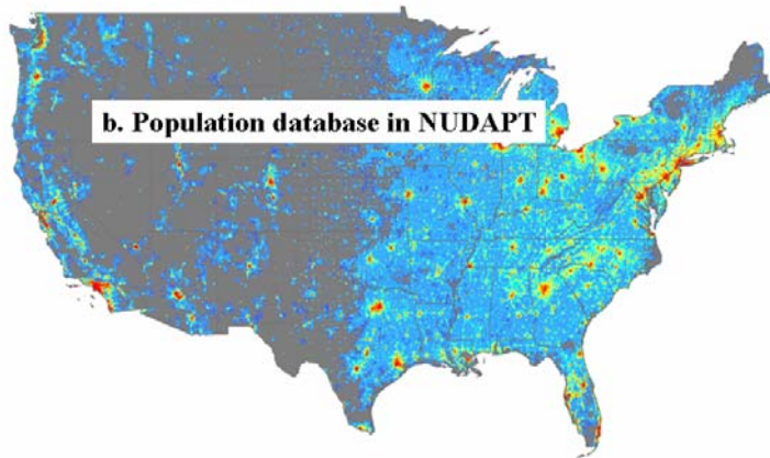
Figure 5: Daytime and nighttime population for (a) central Houston, TX, gridded at 250-m resolution and (b) the CONUS coverage of both day and night population data in NUDAPT. Nighttime maps are derived from Census 2000; and daytime values are based on worker population (processing methodology based on McPherson and Brown, 2003).
