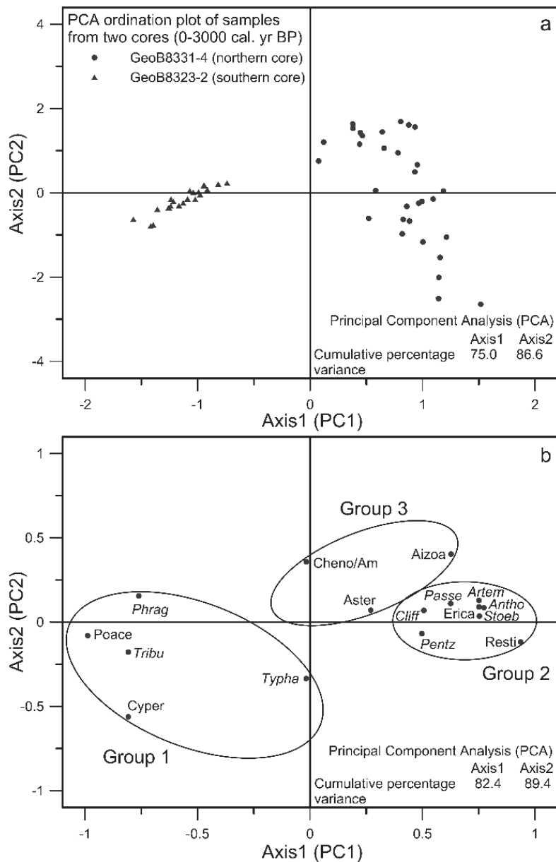
Figure 2.6 (a) PCA ordination plot of the 31 samples from gravity core GeoB8331-4 and 22 samples from gravity core GeoB8323-2 using all pollen and spore taxa. Dots represent samples from core GeoB8331-4 and triangles represent samples from core GeoB8323-2. (b) PCA ordination plot of 16 selected pollen taxa from cores GeoB8331-4 and GeoB8323-2. Group 1: Poace (Poaceae), Cyper (Cyperaceae), Phrag ( Phragmites -type), Typha and Tribu ( Tribulus ). Group 2: Resti (Restionaceae), Erica (Ericaceae), Antho ( Anthospermum ), Stoeb ( Stoebe/Elytropappus -type), Cliff ( Cliffortia ), Passe ( Passerina ), Artem ( Artemisia -type) and Pentz ( Pentzia -type). Group 3: Aizo (Aizoaceae, incl. Mesembryanthemaceae), Cheno/Am (Chenopodiaceae, Amaranthaceae) and Aster (Asteroideae).
