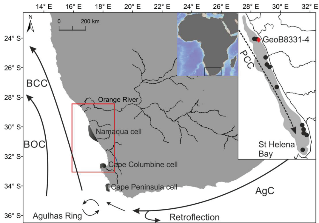
Figure 4.1 Map of the research area showing the locations of 12 multicores (black dots) and the gravity core GeoB8331-4 (red diamond) retrieved from the Namaqualand mudbelt (grey shaded area in the upper right corner) off the west coast of South Africa. The arrows indicate the major oceanic surface current systems: BCC (Benguela Coast Current), BOC (Benguela Ocean Current), AgC (Agulhas Current), PCC (poleward countercurrent). The locations of three main upwelling cells in the southern Benguela region are denoted with black shading: Namaqua cell, Cape Columbine cell and Cape Peninsula cell.
