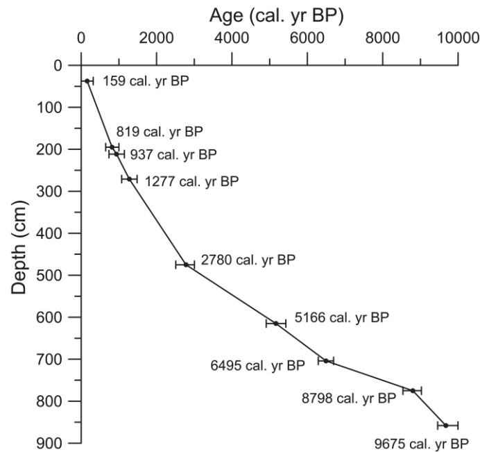
Figure 4.2 Age-depth curve with calculated uncertainty ( 2\sigma ) for the gravity core GeoB8331-4 (Herbert and Compton, 2007; Hahn et al., 2016). The median values of calibrated radiocarbon ages are shown in the figure.
