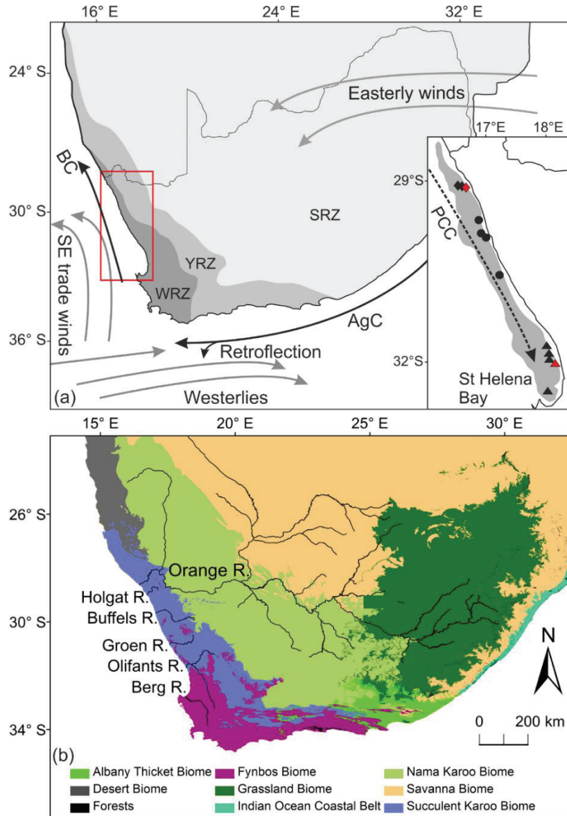
Figure 2.1 Maps of southern Africa showing: (a) modern austral summer atmospheric (gray arrows) and oceanic (black arrows) circulation systems, three rainfall zones of southern Africa are indicated: summer rainfall zone (SRZ), year-round rainfall zone (YRZ) and winter rainfall zone (WRZ). Major representations of oceanic circulation, Benguela Current (BC), Agulhas Current (AgC) are shown. The inset denotes the Namaqualand mudbelt (shading) after Birch et al. (1991), poleward countercurrent (PCC) and multicore locations (diamonds represent samples from the northern mudbelt, dots represent samples from the central mudbelt and triangles represent samples from the southern mudbelt, two gravity cores GeoB8331-4 and GeoB8323-2 are marked in red). (b) Modern vegetation of southern Africa (after Mucina and Rutherford, 2006; Scott et al., 2012), Orange River catchment and main rivers on the west coast.
