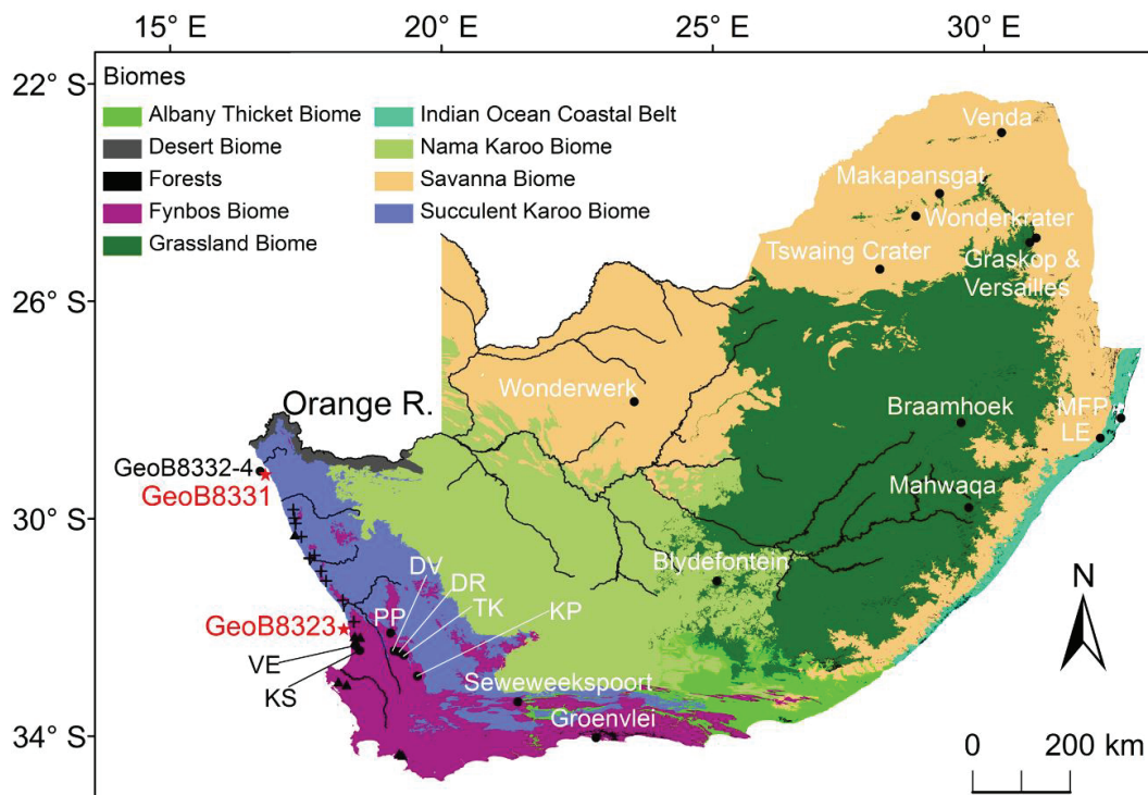
Figure 3.2 Map of southern Africa showing the location of study sites GeoB8331 (gravity core GeoB8331-4 and multicore GeoB8331-2) and GeoB8323 (gravity core GeoB8323-2 and multicore GeoB8323-1) (red stars), as well as gravity core GeoB8332-4 (dot) (Weldeab et al., 2013). Other terrestrial records mentioned in the text (crosses, triangles, and dots) are shown. The crosses denote the sites from Chase and Thomas (2006), the triangles denote the sites from Klein (1991), and the dots denote the sites from a wider area over South Africa (MFP = Mfabeni peatland, LE = Lake Eteza, VE = Verlorenvlei, KS = Klaarfontein Springs, PP = Pakhuis Pass, DV = Driehoek Vlei, DR = De Rif, TK = Truitjes Kraal, KP = Katbakkies Pass). The major biomes of South Africa (Mucina and Rutherford, 2006) are shown.
