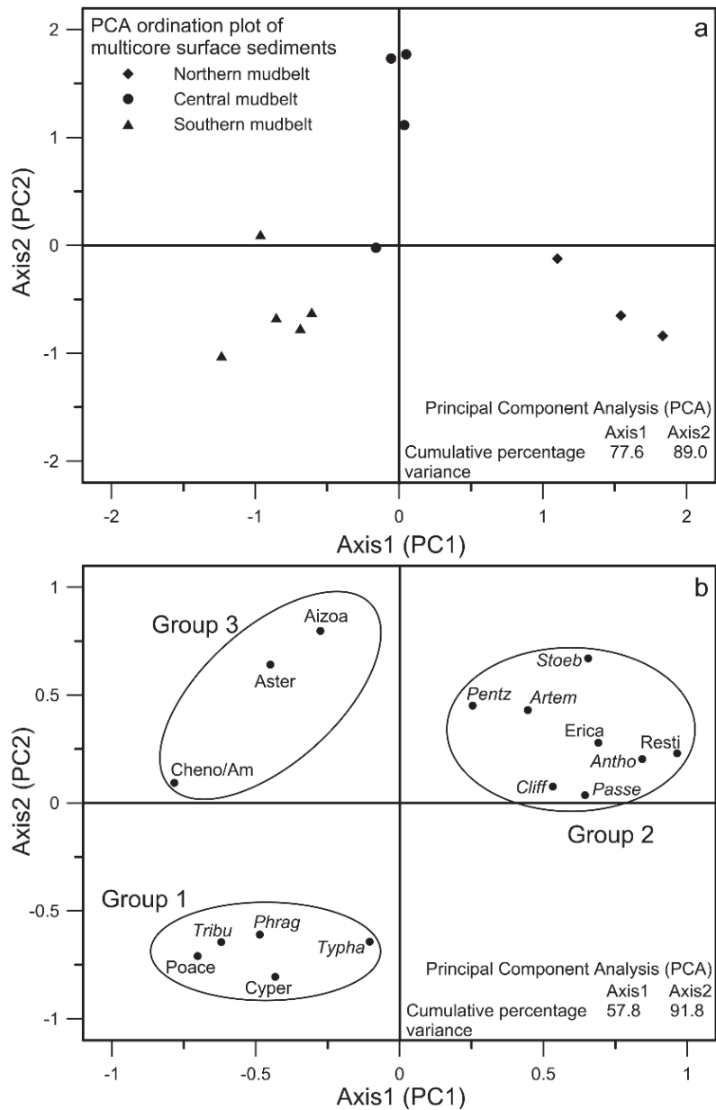
Figure 2.4 (a) PCA ordination plot of the 12 marine surface sediment samples from the Namaqualand mudbelt using all pollen and spore taxa. Diamonds represent samples from the northern mudbelt, dots represent samples from the central mudbelt and triangles represent samples from the southern mudbelt. (b) PCA ordination plot of 16 selected pollen taxa from marine surface sediments from the Namaqualand mudbelt. Group 1: Poace (Poaceae), Cyper (Cyperaceae), Phrag ( Phragmites -type), Typha and Tribu ( Tribulus ). Group 2: Resti (Restionaceae), Erica (Ericaceae), Antho ( Anthospermum ), Stoeb ( Stoebe/Elytropappus -type),
