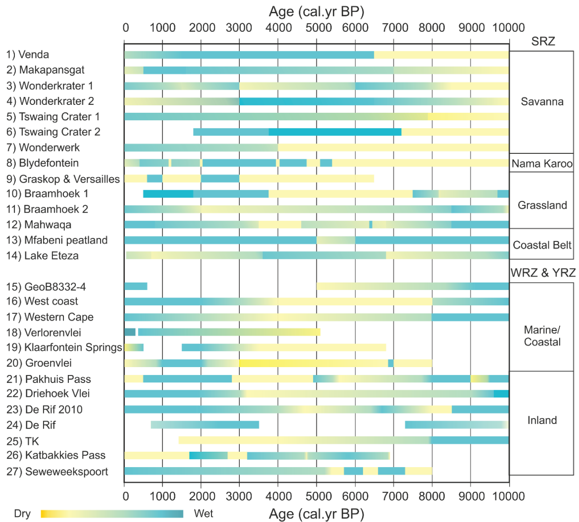
Figure 3.3 Holocene hydrological records from South Africa discussed in the text. This is not an exhaustive data set but includes records covering the whole or at least most period of Holocene. SRZ: (1) Venda (Scott, 1987); (2) Makapansgat (Holmgren et al., 2003); (3) Wonderkrater 1 (Scott et al., 2012); (4) Wonderkrater 2 (Truc et al., 2013); (5) Tswaing Crater 1 (Kristen et al., 2007); (6) Tswaing Crater 2 (Metwally et al., 2014); (7) Wonderwerk (Brook et al., 2010); (8) Blydefontein (Scott et al., 2005); (9) Graskop & Versailles (Bremner et al., 2012); (10) Braamhoek 1 (Norström et al., 2009); (11) Braamhoek 2 (Norström et al., 2014); (12) Mahwaqa (Neumann et al., 2014); (13) Mfabeni peatland (Baker et al., 2014); (14) Lake Eteza (Neumann et al., 2010). WRZ: (15) GeoB 8332-4 (Weldeab et al., 2013); (16) West coast (Chase and Thomas, 2006); (17) Western Cape (Klein, 1991); (18) Verlorenvlei (Meadows et al., 1994, 1996); (19) Klaarfontein Springs (Meadows and Baxter, 2001); (21) Pakhuis Pass (Scott and Woodborne, 2007b); (22) Driehoek Vlei (Meadows and Sugden, 1991); (23) De Rif 2010 (Valsecchi et al., 2013); (24) De Rif (Quick et al., 2011); (25) TK (Truitjes Kraal) (Meadows et al., 2010); (26) Katbakkies Pass (Chase et al., 2015). YRZ: (20) Groenvlei (Martin, 1968); (27) Seweweekspoort (Chase et al., 2013).
