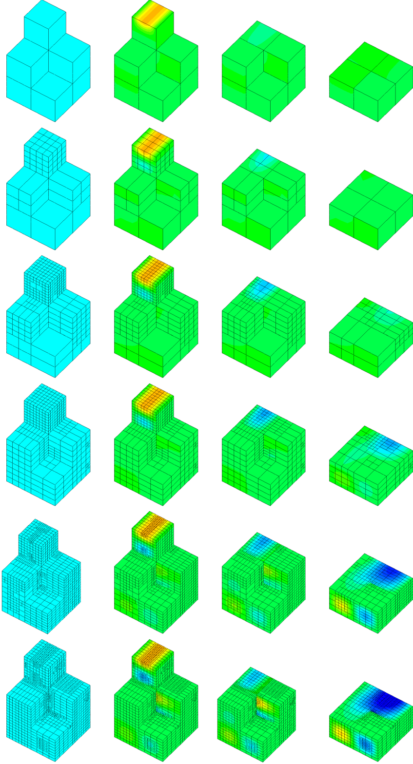
FIGURE 5. Every other iterate (iterates 1,3,5,7,9 and 11) from adaptive algorithm applied to solve the Fichera over problem with the primal formulation. Meshes (left) and the corresponding real part of E_1 are shown.
