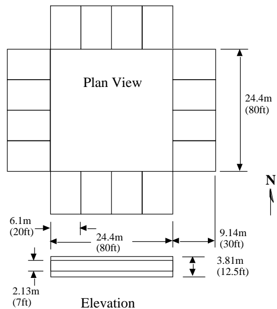
Figure 1. Commercial office building module used in the simulations. Each perimeter zone is partitioned into four offices, each 6.1 m x 9.1 m (20 ft x 30 ft). The core zone has a floor area of 594.6m 2 (6400ft 2 ).
