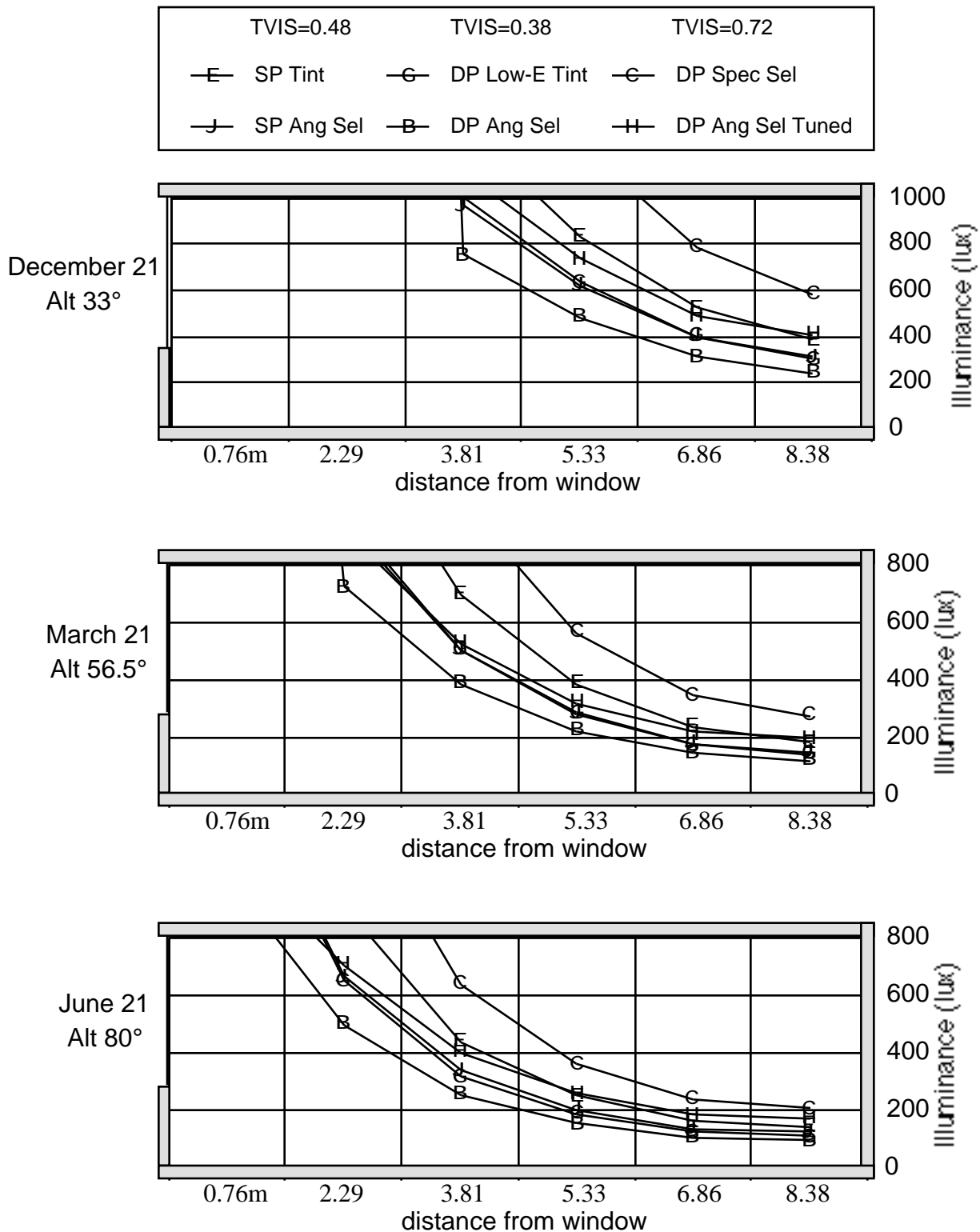
Figure 10. Workplane illuminance distribution with an expanded vertical scale in a south-facing perimeter space at noon with a window-to-wall ratio of 0.56 in Blythe, California.
