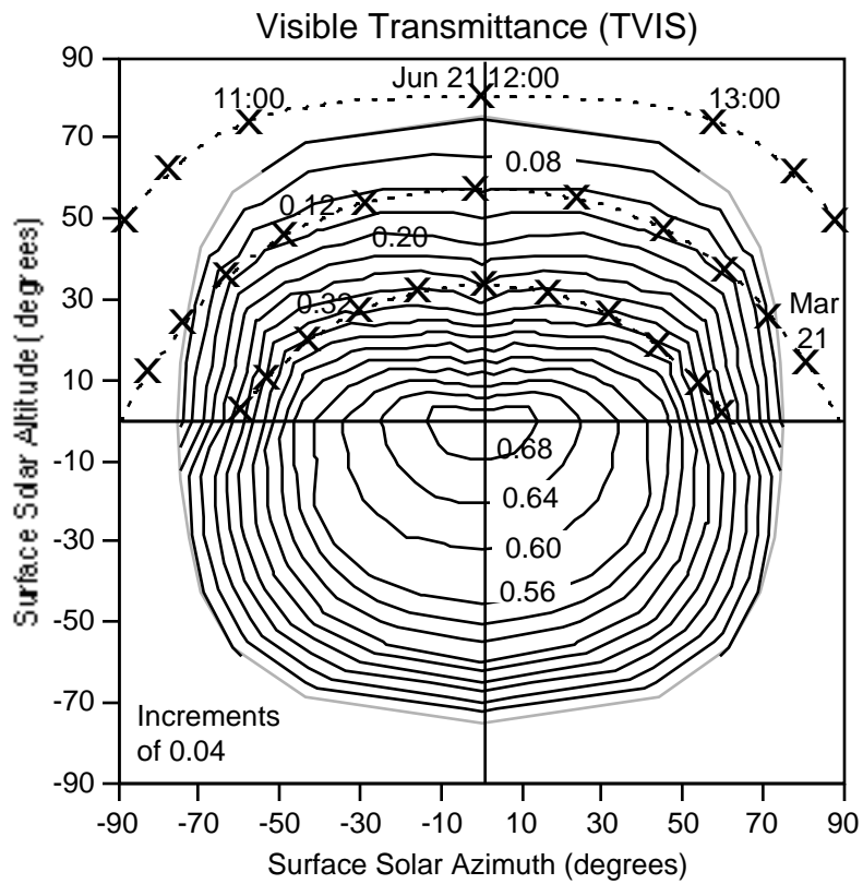
Figure 6. Double Pane Angular Selective Glazing with Tuned TSOL and TVIS Distribution
