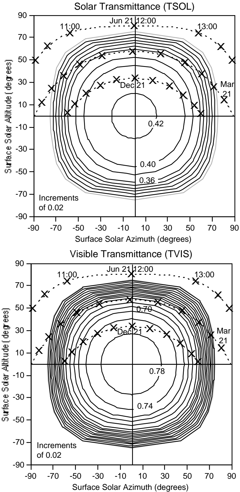
Figure 3. Single Pane Spectrally Selective Glazing TSOL and TVIS Distribution
