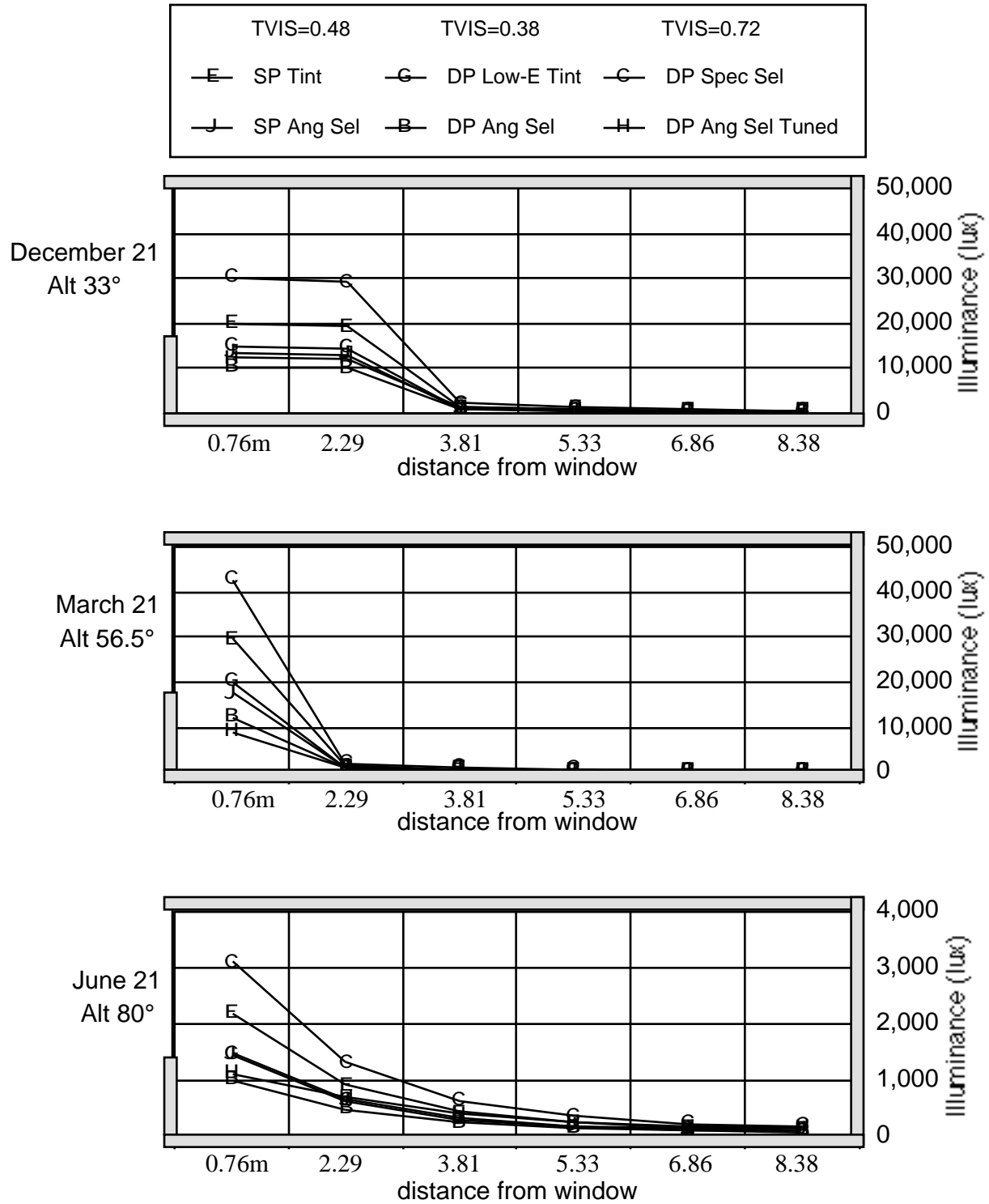
Figure 9. Workplane illuminance distribution in a south-facing perimeter space at noon with a window-to-wall ratio of 0.56 in Blythe, California.
