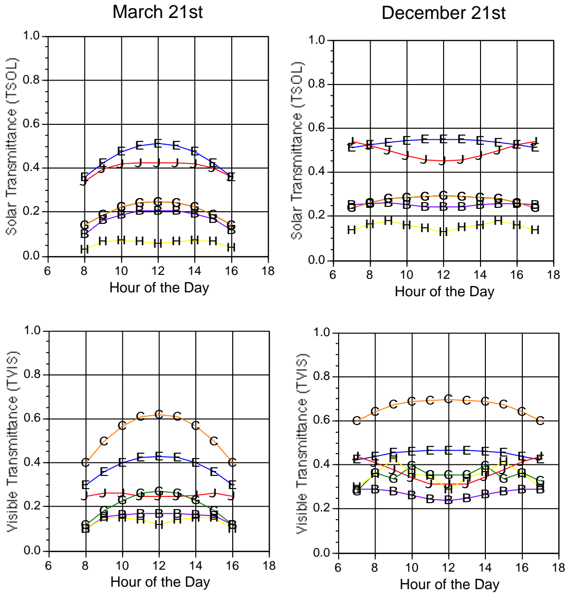
Figure 7. TSOL and TVIS variation during March 21 and December 21 at 33°N latitude for angular selective and conventional windows facing south.
