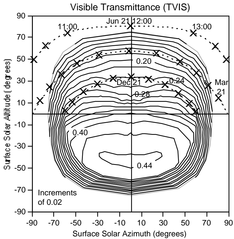
Figure 4. Double Pane Angular Selective Glazing TSOL and TVIS Distribution
