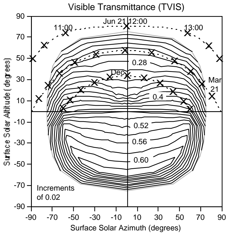
Figure 2. Single Pane Angular Selective Glazing TSOL and TVIS Distribution
