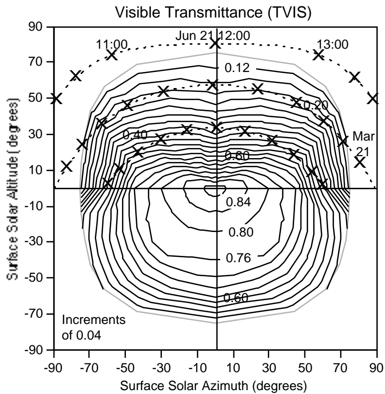
Figure 5. Single Pane Angular Selective Glazing with Tuned TSOL and TVIS Distribution
