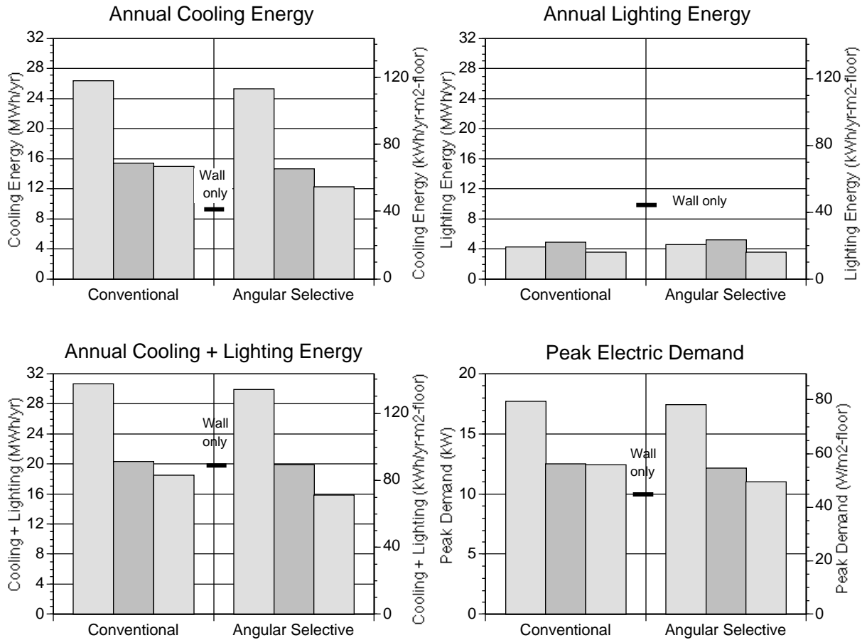
Figure 8. Annual electricity consumption due to cooling (chiller and fans) and lighting, and peak electricity demand for a south-facing perimeter zone in a large prototypical commercial office building module located in Blythe, California. Window-to-wall ratio is 0.56. All systems use continuous dimming daylight controls and a lighting power density of 16.1 W/m 2 (1.5 W/ft 2 ).
