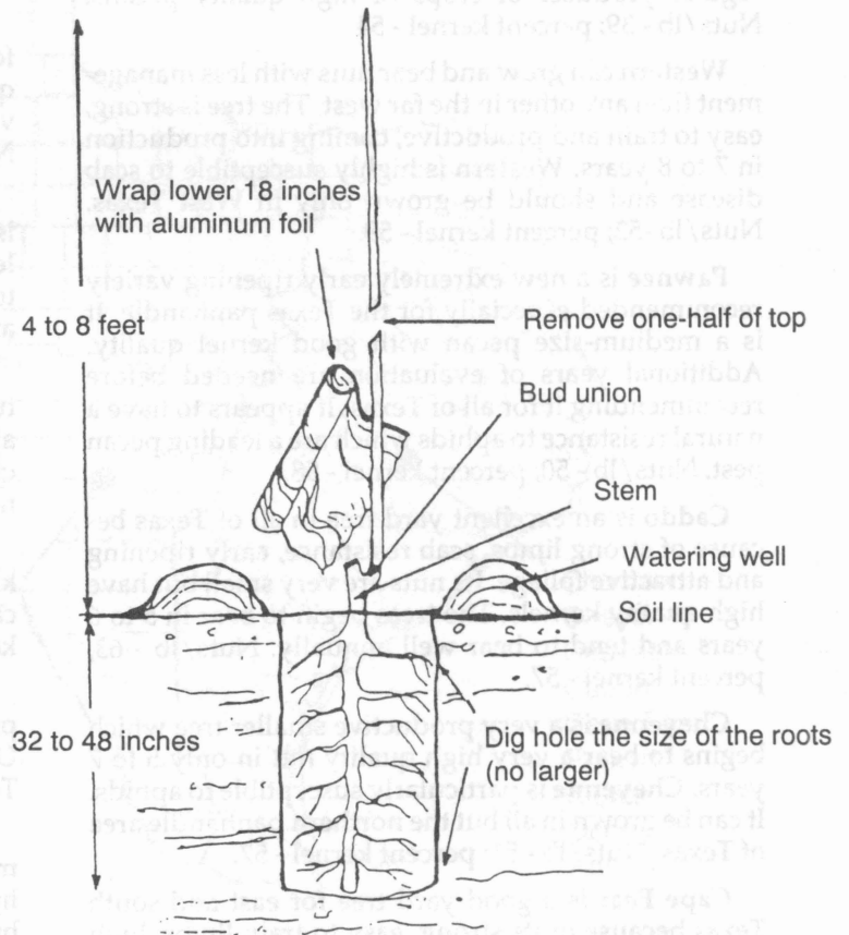
Figure 2. How to properly plant a pecan tree.
