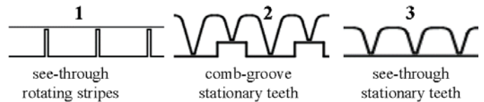
FIGURE 5. INVESTIGATED LABYRINTH SEAL TYPES.
