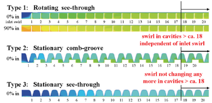
FIGURE 9. PATTERN OF THE CIRCUMFERENTIAL FLOW FOR THE THREE INVESTIGATED LABYRINTH TYPES.
