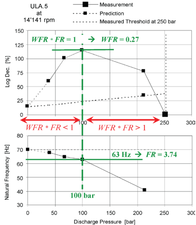
FIGURE 19. MEASURED NATURAL FREQUENCY AND DAMPING FOR CONFIGURATION ULA.5. (FIGURE 9, BAUMANN, 1999)
