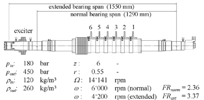
FIGURE 18. HIGH PRESSURE COMPRESSOR ROTOR SHOWING TWO POSSIBLE BEARING LOCATIONS (NORMAL AND EXTENDED) AND OPERATING PARAMETERS.
