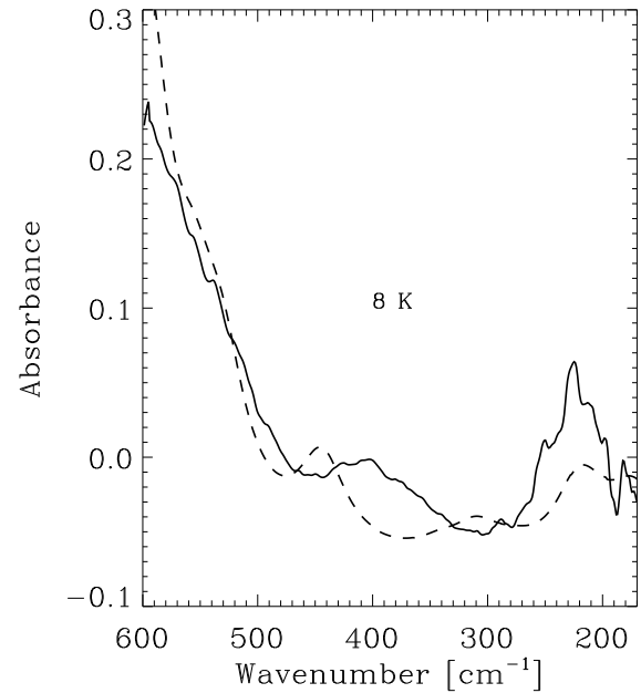
Fig. 9. Infrared spectra of an H 2 O:NH 3 3:1 ice mixture in the far-IR region at 8 K (solid line). The dashed line represents the calculated spectrum of an ice mixture of the same composition.
