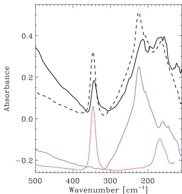
Fig. 3. Infrared spectra of an H 2 O:CH 3 OH 1:1 ice mixture in the far-IR region at 130 K (black solid line) along with the spectra of pure water (blue solid line) and methanol (red solid line) ices of the same thicknesses as that of each species in the ice mixture. Pure ice spectra are shifted for clarity. The dashed line is the sum of the two pure ice spectra.
