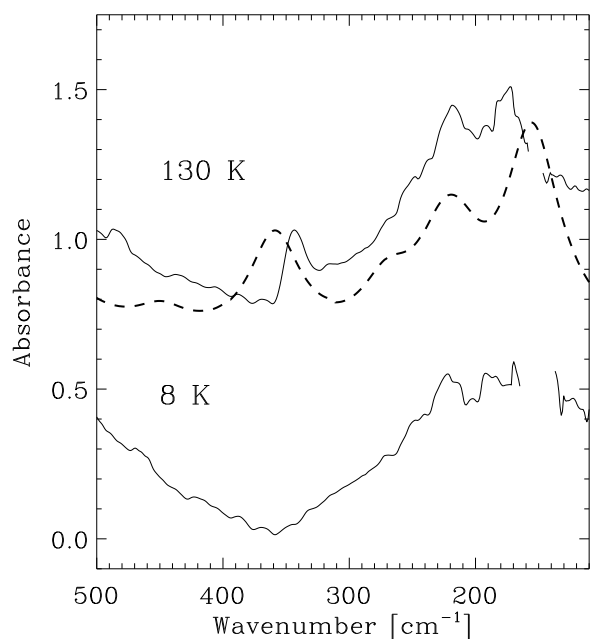
Fig. 4. Infrared spectra of an H 2 O:CH 3 OH 3:1 ice mixture in the far-IR region at 8 K and annealed at 130 K (solid lines). Spectra are offset for clarity. Spectral regions with high noise are not shown. The dashed line represents the calculated spectrum of an ice mixture of the same composition, which is in better agreement with the spectrum of the annealed ice.
