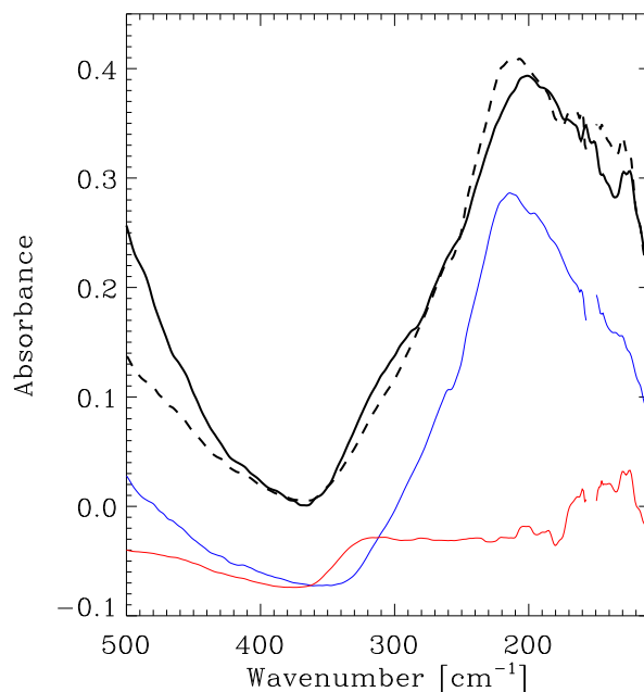
Fig. 2. Infrared spectra of an \text{H}_2\text{O}:\text{CH}_3\text{OH} 1:1 ice mixture in the far-IR region at 8 K (black solid line) along with the spectra of pure water (blue solid line) and methanol (red solid line) ices of the same thicknesses as that of each species in the ice mixture. Pure ice spectra are shifted for clarity. The dashed line is the sum of the two pure ice spectra. A small region around 150 \text{ cm}^{-1} is not shown because of the high noise collected at those frequencies.
