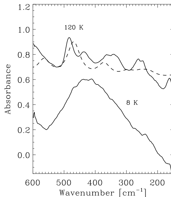
Fig. 11. Infrared spectra of an \text{H}_2\text{O}:\text{NH}_3 1:3 ice mixture in the far-IR region at 8 K and annealed at 120 K (solid lines). The \text{H}_2\text{O}:\text{NH}_3 ratio of the annealed mixture is greater than 1 due to ammonia desorption (see text). Spectra are offset for clarity. The dashed line represents the calculated spectrum of an ice mixture of the same composition, which is in better agreement with the spectrum of the annealed ice.
