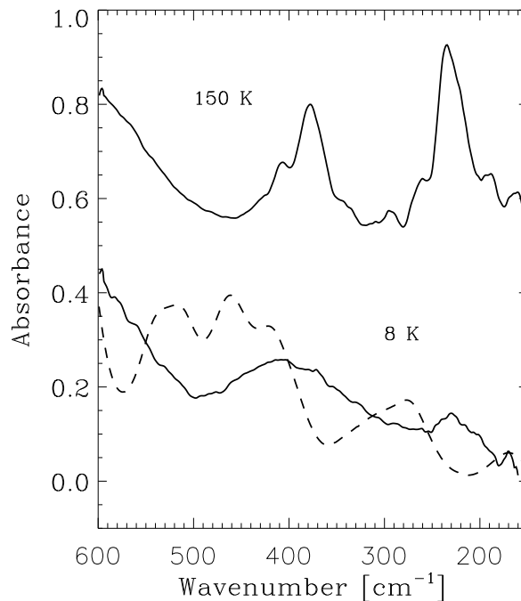
Fig. 6. Infrared spectra of an \text{H}_2\text{O}:\text{NH}_3 1:1 ice mixture in the far-IR region at 8 K and annealed to 150 K (solid lines). The \text{H}_2\text{O}:\text{NH}_3 ratio of the annealed mixture is greater than 1 because of ammonia desorption (see text). Spectra are offset for clarity. The dashed line represents the calculated spectrum of an ice mixture of the same composition.
