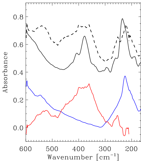
Fig. 8. Infrared spectra of an H 2 O:NH 3 ice mixture deposited with a 1:1 ratio in the far-IR region at 150 K (black solid line) along with the spectra of pure water (blue solid line) and ammonia (red solid line) ices of the same thicknesses as that of each species in the deposited ice mixture. Pure ice spectra are shifted for clarity. The dashed line is the sum of the two pure ice spectra.
