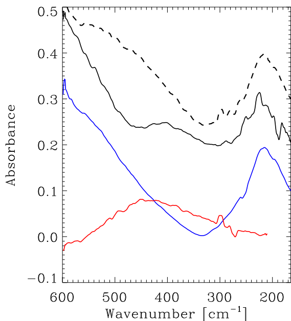
Fig. 10. Infrared spectra of an \text{H}_2\text{O}:\text{NH}_3 3:1 ice mixture in the far-IR region at 8 K (solid line) along with the spectra of pure water (blue solid line) and ammonia (red solid line) ices of the same thicknesses as that of each species in the ice mixture. Pure ice spectra are shifted for clarity. The dashed line represents the sum of the two pure ice spectra.
