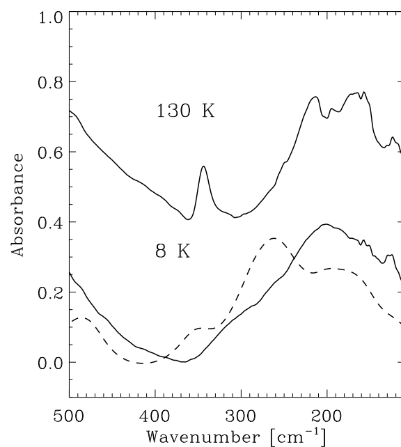
Fig. 1. Infrared spectra of an H 2 O:CH 3 OH 1:1 ice mixture in the far-IR region at 8 K and 130 K (solid lines). Spectra are offset for clarity. The dashed line represents the calculated spectrum of an ice mixture of the same composition.
