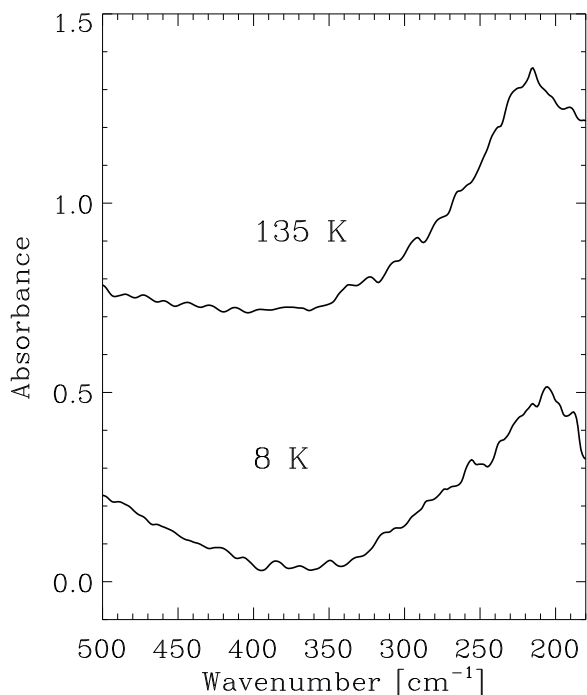
Fig. 5. Infrared spectra of an \text{H}_2\text{O}:\text{CH}_3\text{OH} 10:1 ice mixture in the far-IR region at 8 K and 135 K. Spectra are offset for clarity. The spectral window is narrower than in Figures 1 and 4 because of elevated noise in the low-frequency region of the spectrum.
