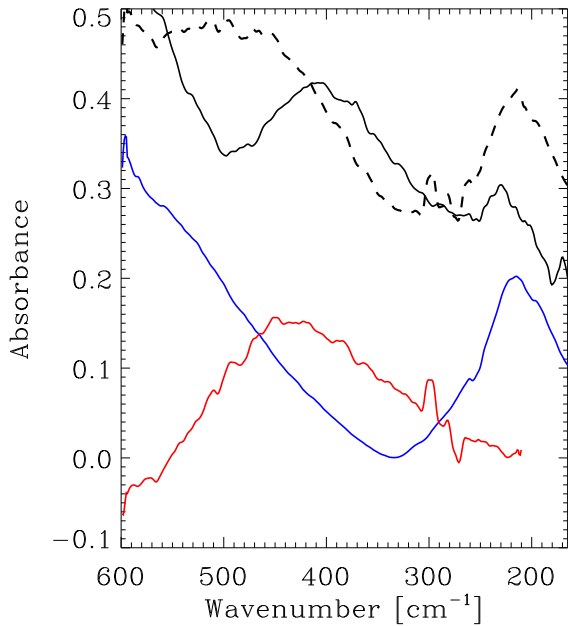
Fig. 7. Infrared spectra of an H 2 O:NH 3 1:1 ice mixture in the far-IR region at 8 K (black solid line) along with the spectra of pure water (blue solid line) and ammonia (red solid line) ices of the same thicknesses as that of each species in the ice mixture. Pure ice spectra are shifted for clarity. The dashed line is the sum of the two pure ice spectra.
