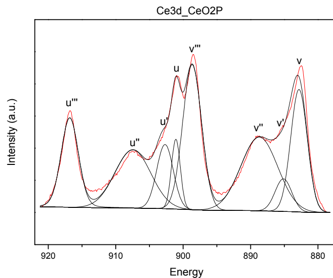
Figure A1. Deconvolution of the Ce3d XPS spectra of one ceria catalyst (Ce-P). The Ce 3d region shows a complex spectrum, which can be decomposed in eight contributions: v, u (Ce (3d 9 4f 2 ) O (2p 4 )) and v''', u''' ((Ce (3d 9 4f 1 ) O (2p 5 )); v''', u''' (final state of Ce (3d 9 4f 0 ) O (2p 6 )) assigned to Ce 4+ ; v', u' (Ce (3d 9 4f 1 ) O (2p 6 )) assigned to Ce 3+ as a consequence of the hybridization between the Ce 4f levels and the O 2p states.
