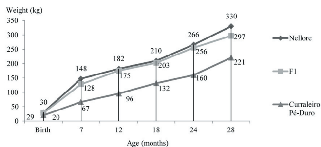
Figure 1 - Growth performance of Nellore, F_1 , and Curraleiro Pé-Duro progenies at different ages.
