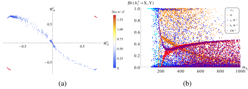
Figure 1: Correlation of g_{h_i^\pm W^\mp Z} with \mathcal{R}_{i2}^C and \mathcal{R}_{i4}^C (a) and two-body decay branching fractions (b) [10].
