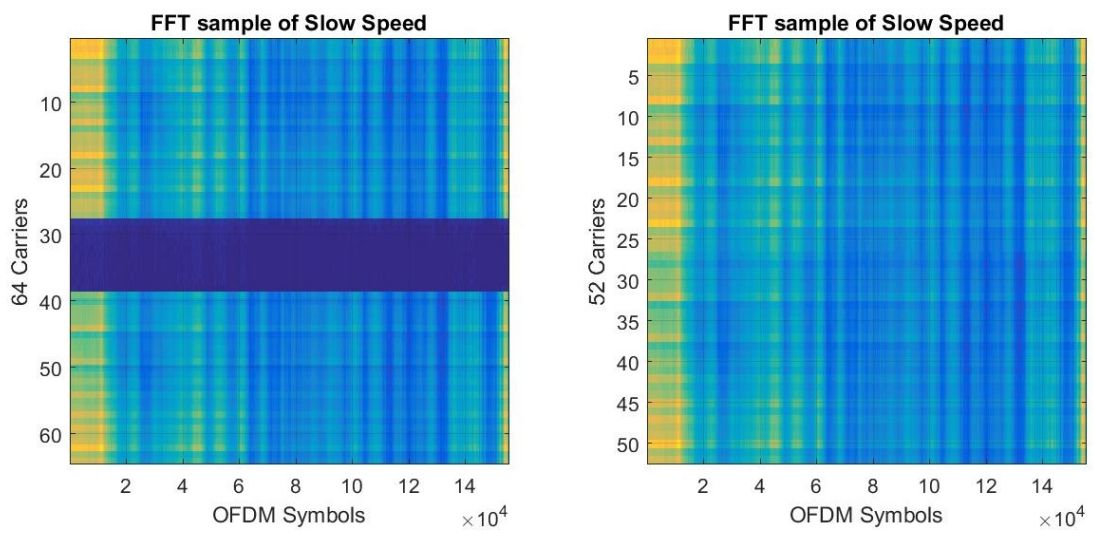
Figure 11: FFT sample of slow speed exploited from one subject before and after removing virtual sub carriers.
