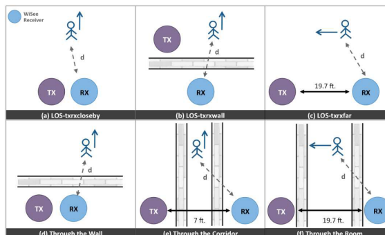
Figure 3: WiSee gesture recognition scenario [3].
