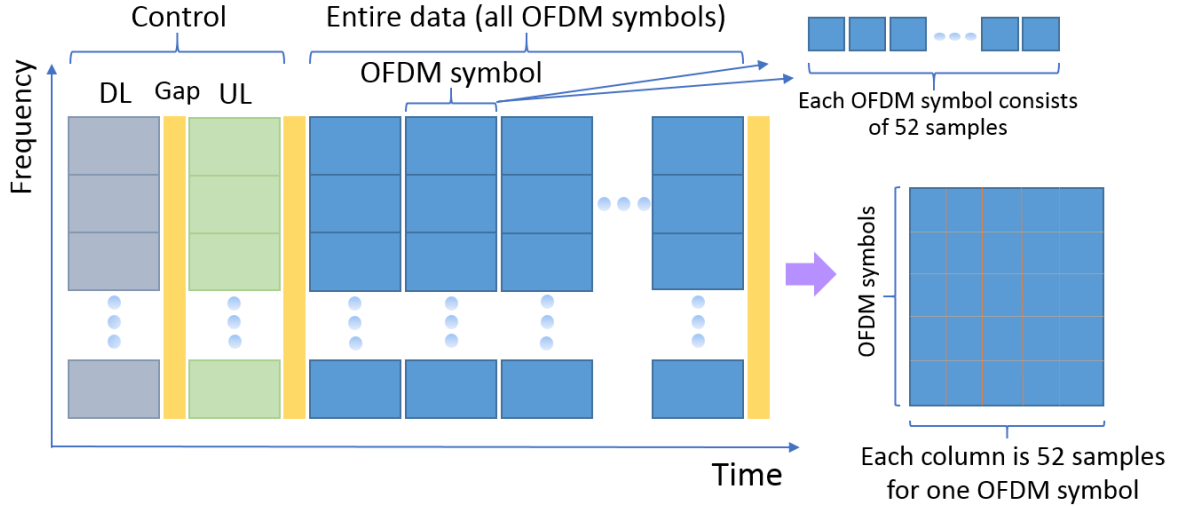
Figure 10: OFDM carriers and symbols as transmitted data in 5G prototype system.
