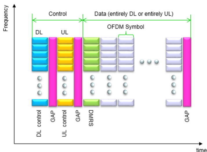
Figure 7: 5G frame structure [6].
