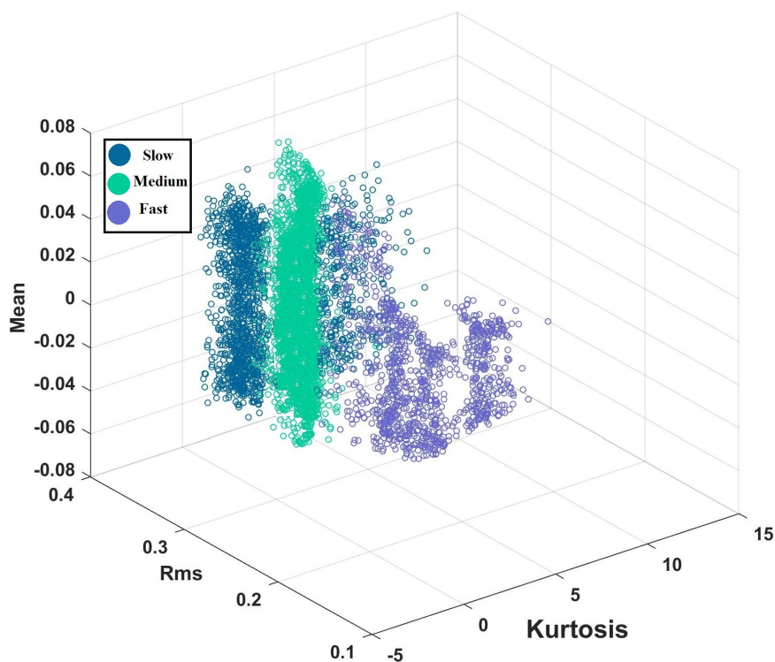
Figure 17: 3D plot of three selected features through all speeds for the best case (26 carriers). It reveals that beside the slight interference between slow, medium and fast speed, they are well distinguished.
