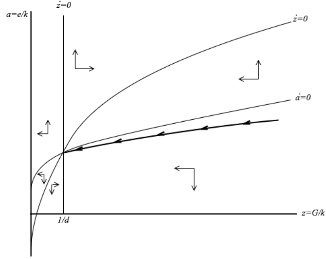
Figure 3.4: Transitional dynamics of the model when the two equilibria have merged into one.
