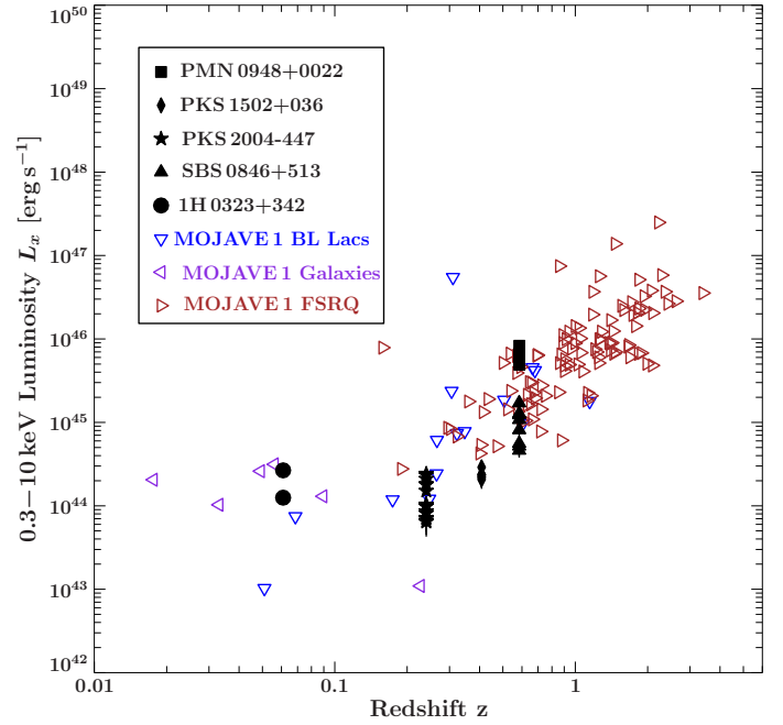
Fig. 8. Comparison of (0.3–10) keV X-ray luminosity L_X as a function of redshift z for the MOJAVE 1 sample (open symbols) and \gamma -NLS1 sources (black filled symbols) discussed in this paper.
