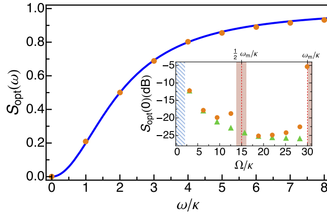
Figure 2. Squeezing spectrum. The full, blue line represents the best squeezing spectrum of the OM cavity, according to the analytical prediction from model (1), for \Omega/\kappa = 4\pi , \Delta/\kappa = -2 , and n_T = 0 . Orange symbols denote the results of numerical simulations of the complete optomechanical problem for the same parameters as in Fig. 1, with \Delta/\kappa = -2 (close below point (b) in Fig. 1; \mu = 0.837 ). The inset shows the dependence of the numerically obtained optimal squeezing on the modulation frequency \Omega , of both superconducting circuit cavities (green diamonds) and optomechanical cavities (orange circles). Parameters as in Fig. 1. Within the left shaded region the mechanism proposed here does not work (a minimum modulation frequency, around \Omega/\kappa = 2\pi , is needed), while in the middle and right ones it does not only for the optomechanical cavity: the rightmost orange circle corresponds to \Omega = 29.9\kappa , slightly less than the mechanical resonance frequency \omega_m = 30\kappa ; for \Omega = \omega_m the effect is completely lost, while for \Omega > \omega_m the scenario completely changes and a different description is needed.
