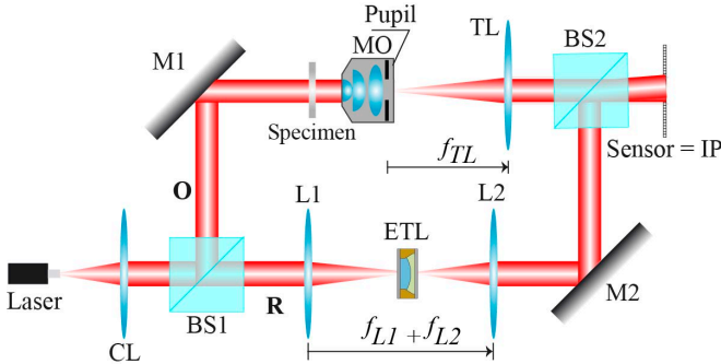
Fig. 1 Proposed set-up to provide PSI using an electronically tunable lens (ETL), which is inserted at the common focal plane of an afocal relay system. CL, collimating lens; BS1 and BS2, are cubes beamsplitters; O, object wave; R, reference wave; M1 and M2, are mirrors; L1 and L2, converging lenses. The microscope objective MO and a tube lens TL operated in telecentric configuration.
