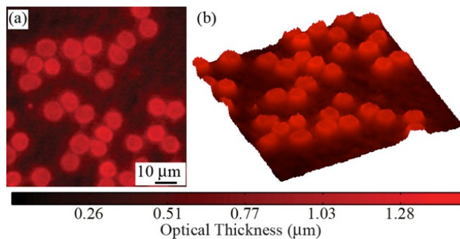
Fig. 6 QPI of human RBCs via PSI-DHM by using ETL as phase shifting device. Panel (a) is the recovered image in terms of optical thickness and panel (b) is its 3D view.
