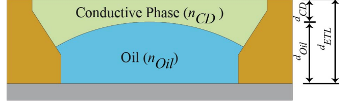
Fig. 2 Electronically tunable lens (ETL) schematics. In green, the conductive phase with refraction index n_{CD} and in blue the oil phase with refraction index n_{Oil} . d_{ETL} is the total thickness of the ETL, d_{Oil} and d_{CD} are thicknesses at the center of the ETL.
