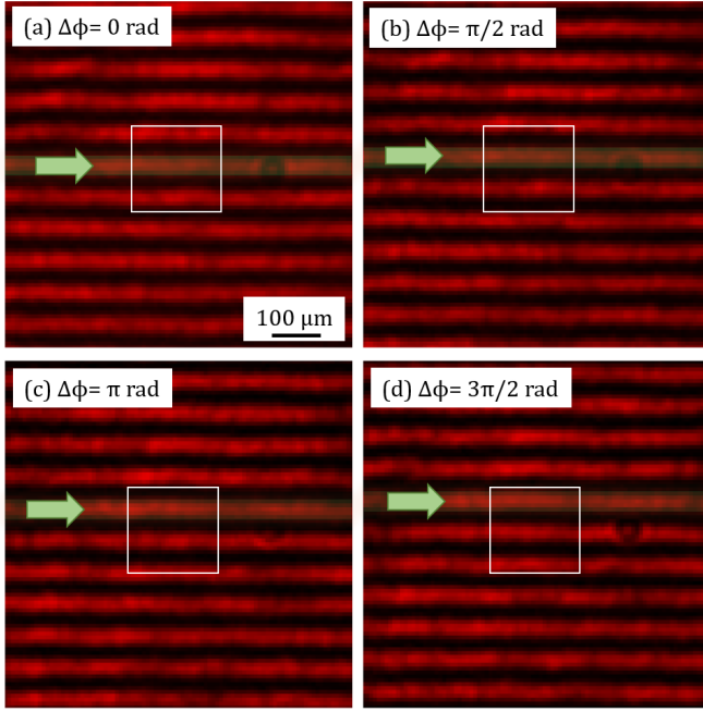
Fig. 3 Experimental holograms as an ETL is used as phase-shifting device. The arrow marks a given fringe as it is moved in regard with the fixed square.
