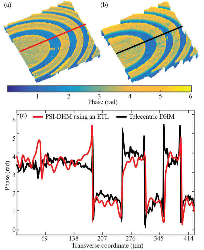
Fig. 4. PSI-DHM v.s. Off-axis telecentric DHM. (a) QPI of a Fresnel's lens by PSI-DHM; (b) QPI of the same Fresnel's lens by off-axis telecentric DHM and (c) profiles along the lines of panels (a) and (b).
