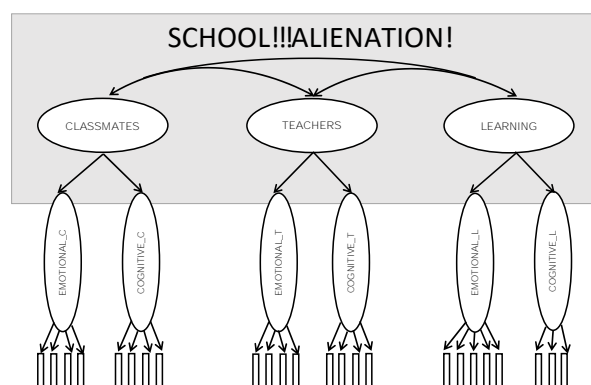
Figure 1. First-order one-factor (Model 1), second-order with three facets included (Model 2), hypothesized first-order three-factor (Model 3), and second-order with six facets included (Model 4) models potentially underlying the SALS.
