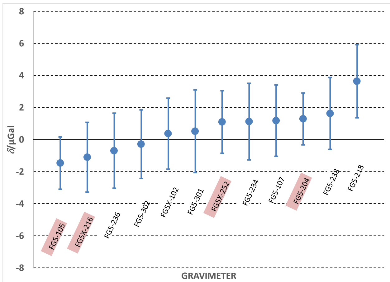
Figure 3. Initial biases \delta of the gravimeters from the initial weighted LSA. Gravimeters of NMI/DIs are highlighted in pink. The error bars are the expanded standard uncertainties ( k=2 ) from the weighted LSA and are listed in Table 6.
