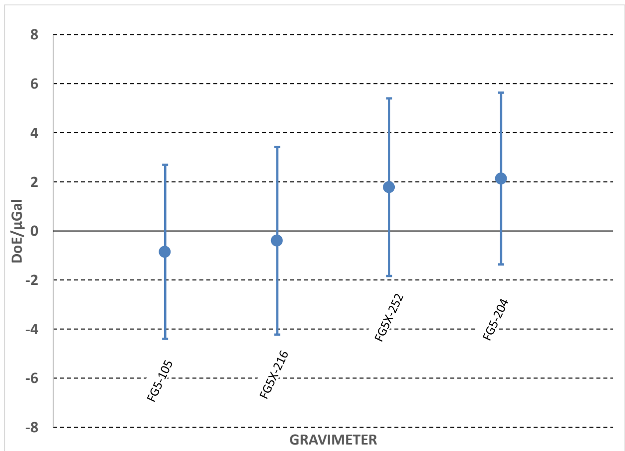
Figure 4. Official DoE results of the NMI/DI gravimeters participating in SIM.M.G-K1. The error bars represent the expanded uncertainties ( U_{DoE} ) of the DoE at 95% confidence.
