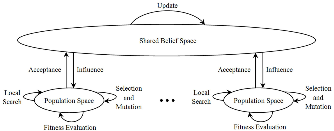
Figure 2.1: H-MPCA Architecture [Raeesi and Kobti, 2013]
