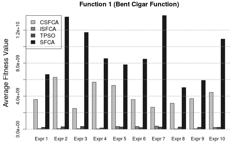
Figure 6.1: Average fitness values for Function 1 with 10 dimensions
