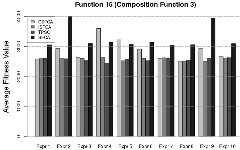
Figure 6.30: Average fitness values for Function 15 with 30 dimensions
