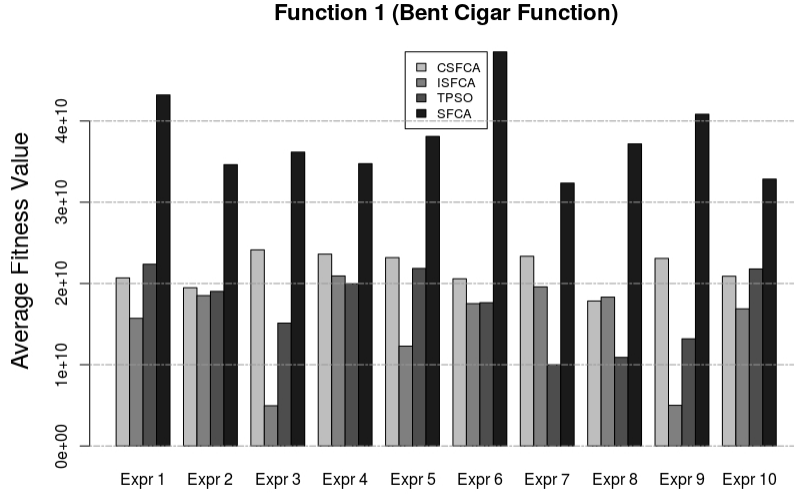
Figure 6.2: Average fitness values for Function 1 with 30 dimensions
