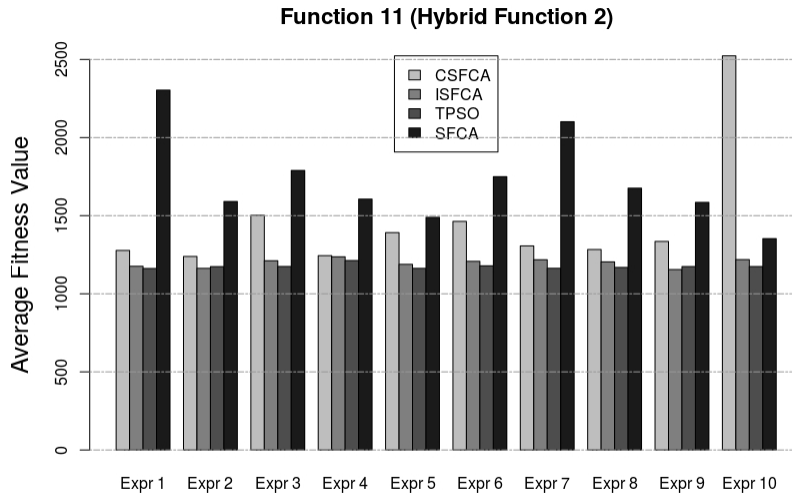
Figure 6.22: Average fitness values for Function 11 with 30 dimensions
