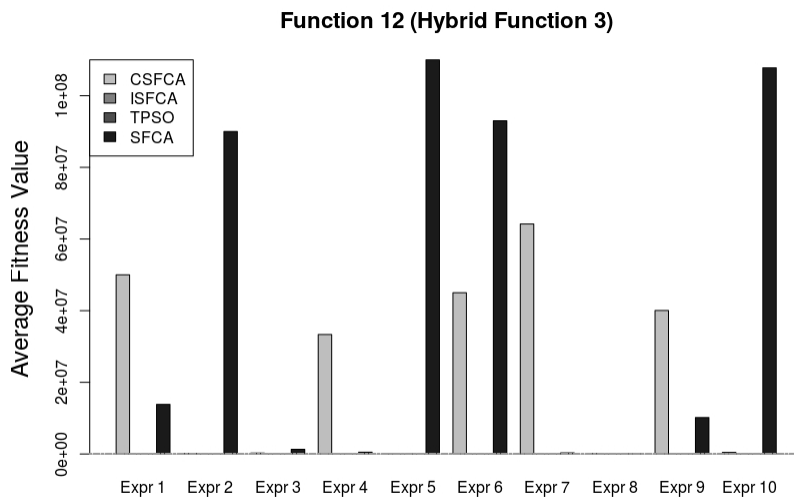
Figure 6.24: Average fitness values for Function 12 with 30 dimensions
