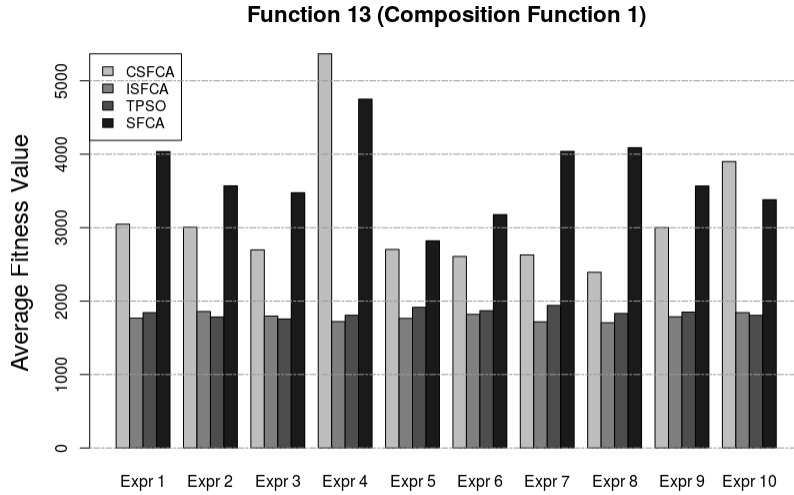
Figure 6.26: Average fitness values for Function 13 with 30 dimensions
