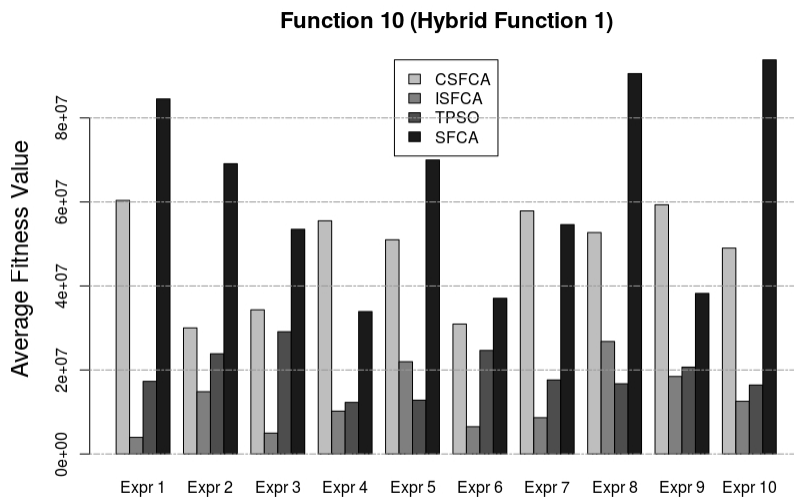
Figure 6.20: Average fitness values for Function 10 with 30 dimensions
