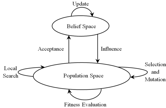
Figure 3.1: Cultural Algorithms [Raeesi and Kobti, 2013]
