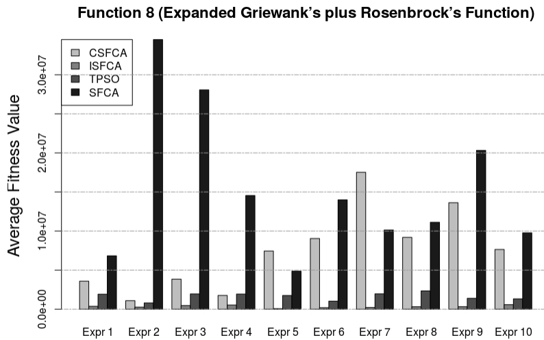
Figure 6.16: Average fitness values for Function 8 with 30 dimensions
