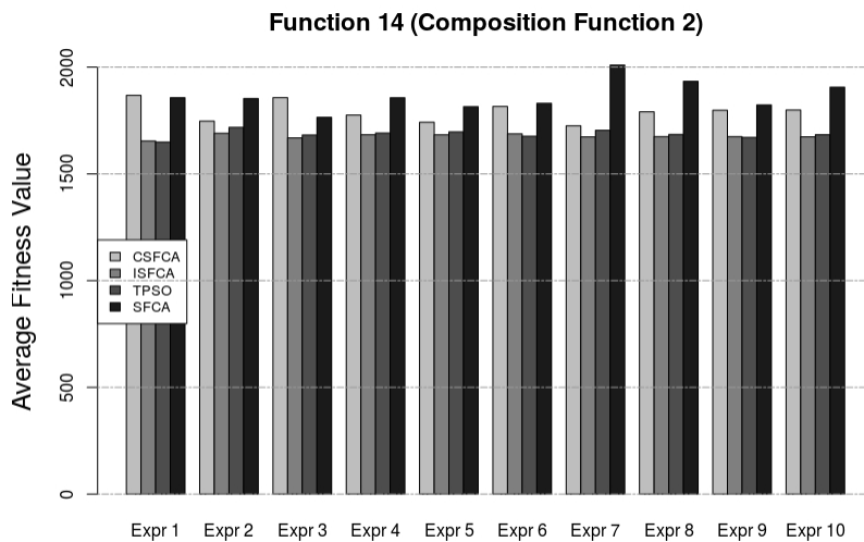
Figure 6.28: Average fitness values for Function 14 with 30 dimensions
