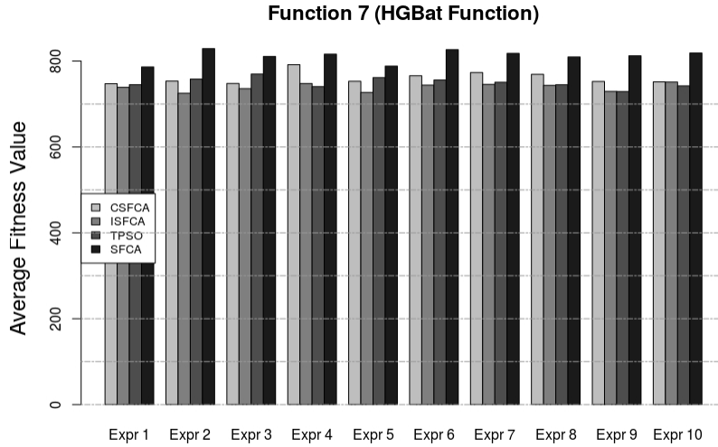
Figure 6.14: Average fitness values for Function 7 with 30 dimensions
