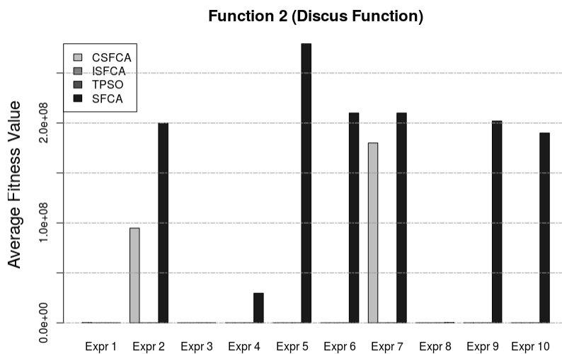
Figure 6.4: Average fitness values for Function 2 with 30 dimensions
