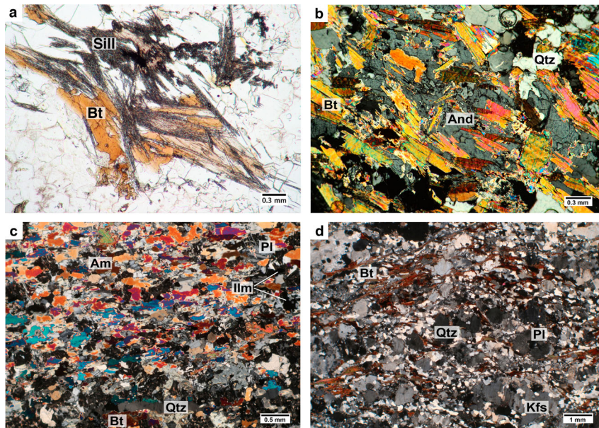
Figure 4. Microphotographs of selected metamorphic lithologies from VMP host rocks. (a) Fibrolitic sillimanite aggregates are observed in the paragneiss residuum of stromatic metatexite migmatite find in proximity to the contact with the VMP; (b) Andalusite and granoblastic quartz are features of the Kinzigite formation paragneiss highlighted in this enlargement. (c) Medium-grained amphibolite in which a continuous foliation is defined by Am and Qtz-Pl domains; (d) Medium-grained orthogneiss from the Strona-Ceneri Zone dominated by a Kfs-Pl-Qtz mineralogy in which biotite marks a weakly developed foliation.
