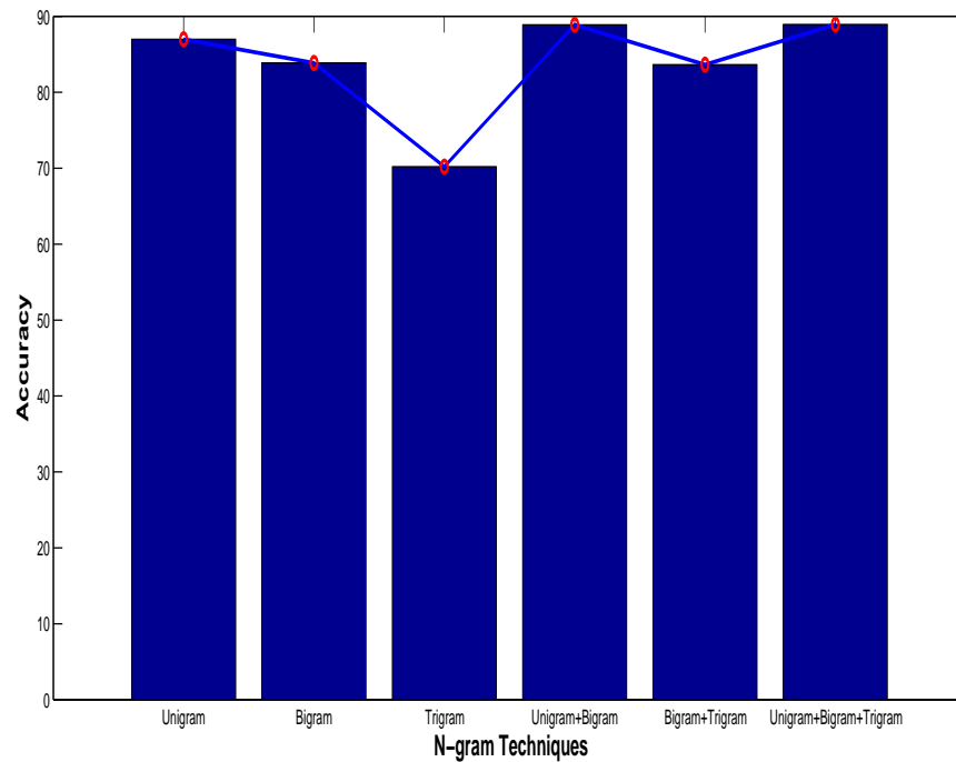
Figure 4.4: Comparison of Accuracy values of different n-gram technique using SVM
