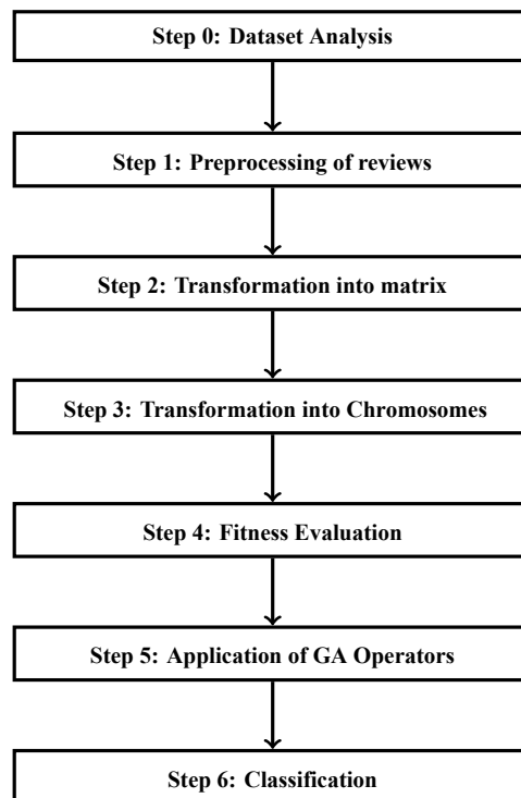
Figure 5.3: Proposed approach for Classification using GA classifier
