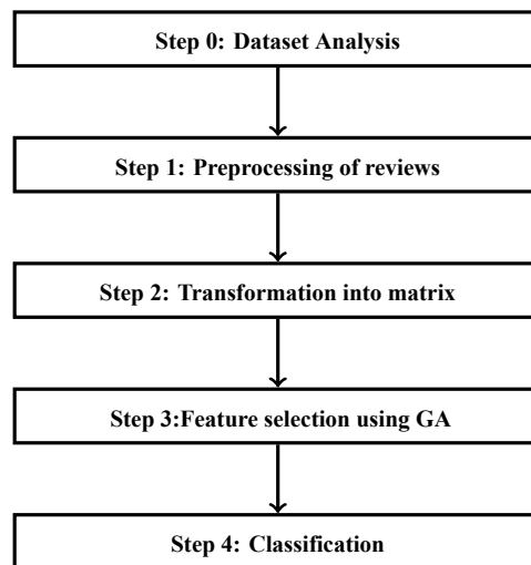
Figure 5.4: Diagrammatic view of the proposed approach using Neuro - GA classifier
