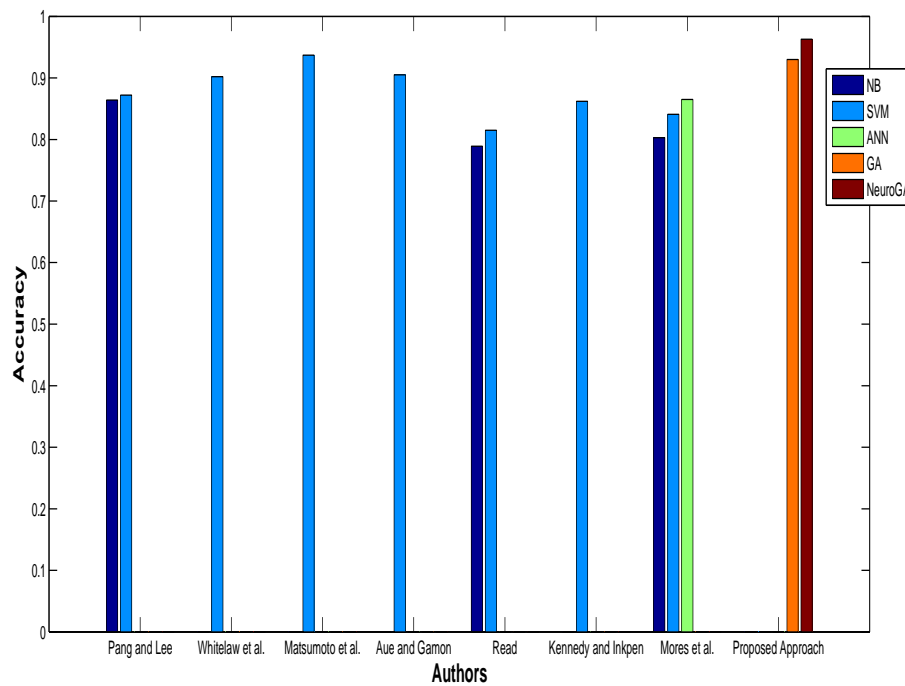
Figure 5.6: Comparison of accuracy values of obtained by different authors on Polarity dataset
