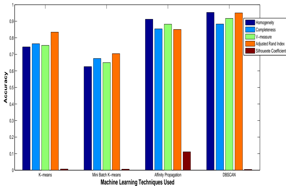
Figure 7.2: Comparison of results obtained using proposed approach
