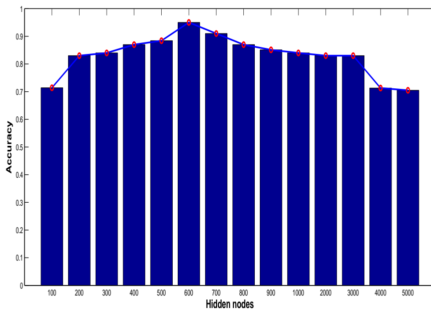
Figure 6.2: Comparison of accuracy values of using different hidden nodes for ANN for IMDb dataset
