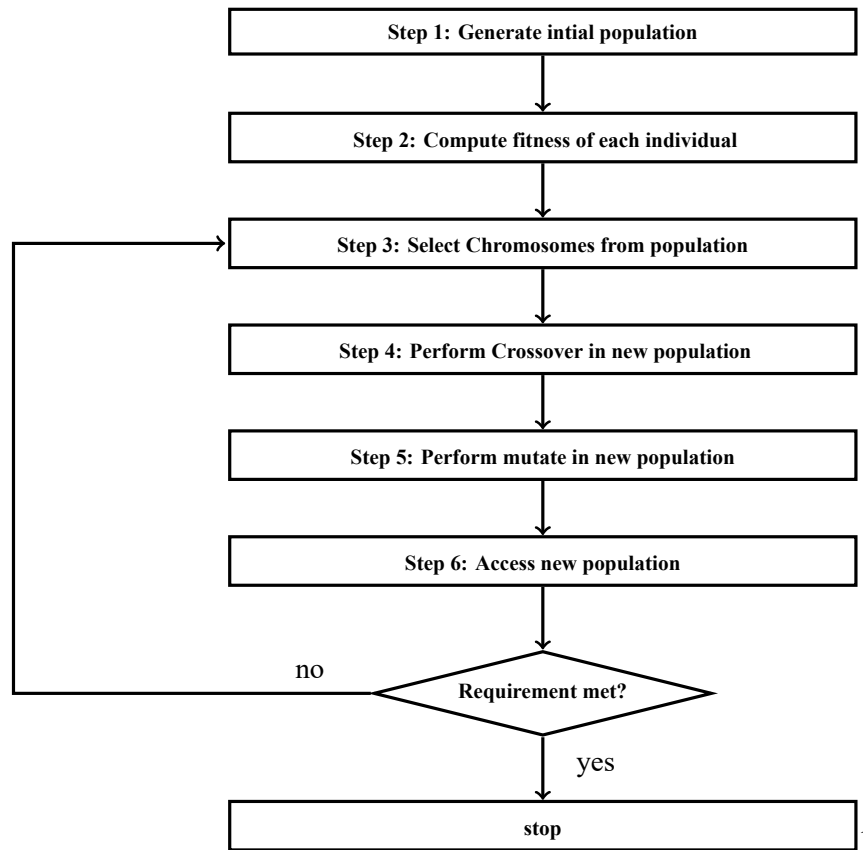
Figure 5.1: Proposed approach for Classification using GA classifier
