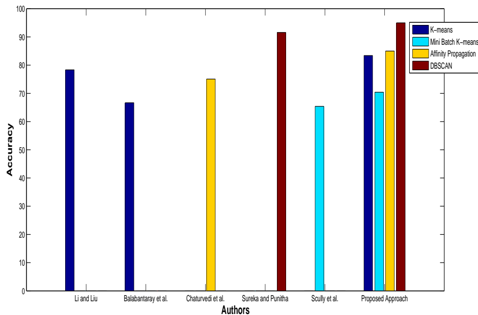
Figure 7.3: Comparison of obtained results with result obtained by other authors
