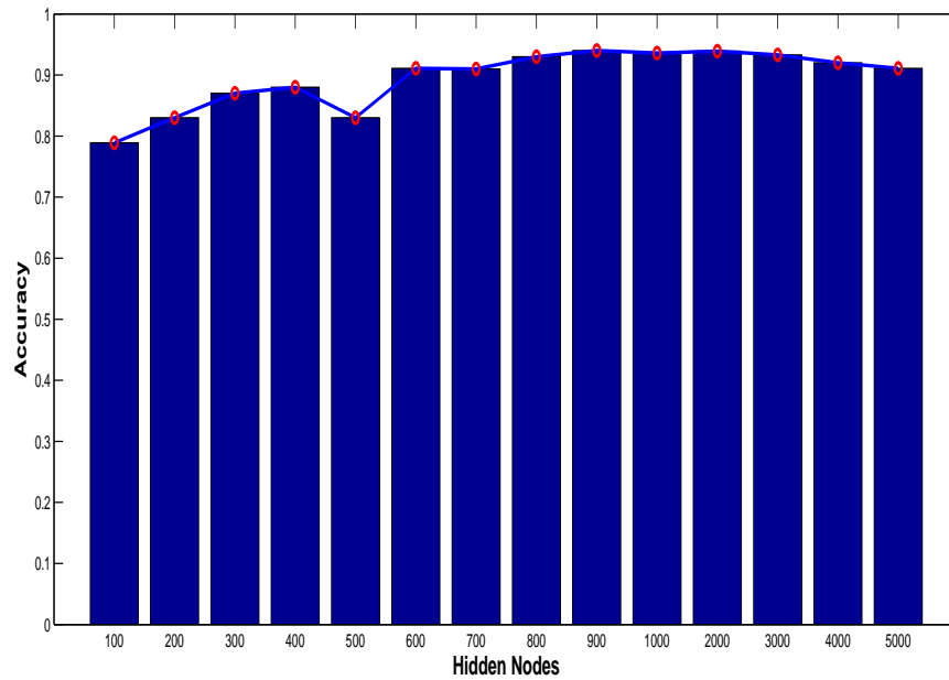
Figure 5.5: Comparison of accuracy values of using different hidden nodes for ANN
