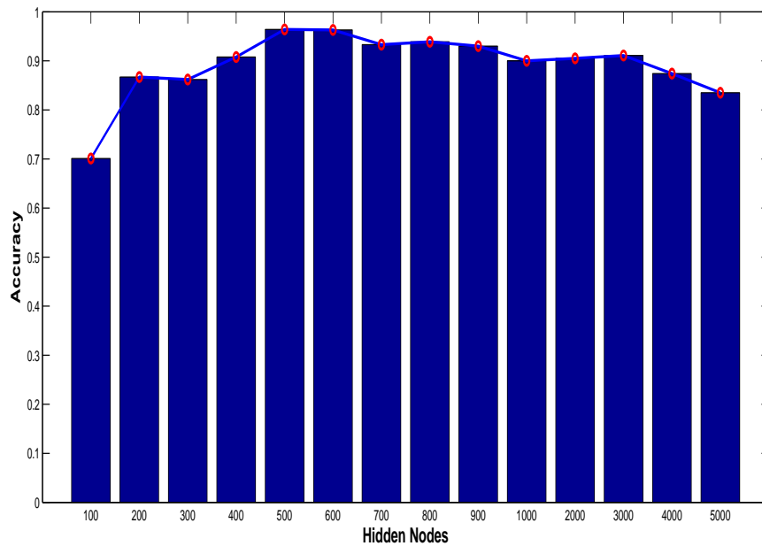
Figure 6.3: Comparison of accuracy values of using different hidden nodes for ANN for polarity dataset
