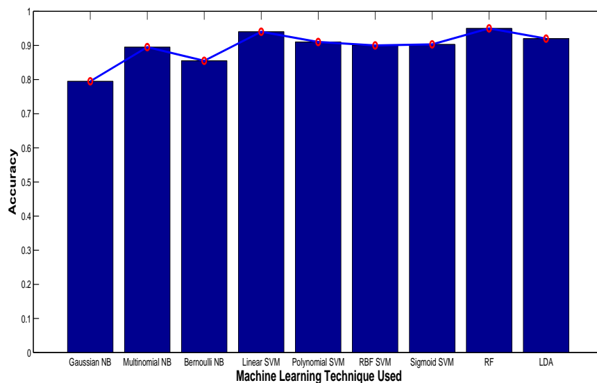
Figure 3.3: Comparison of Accuracy values of Proposed MLTs using polarity dataset
