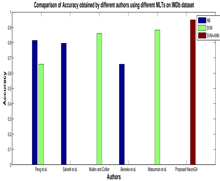
Figure 6.4: Comparison of accuracy values of obtained by different authors on IMDb dataset
