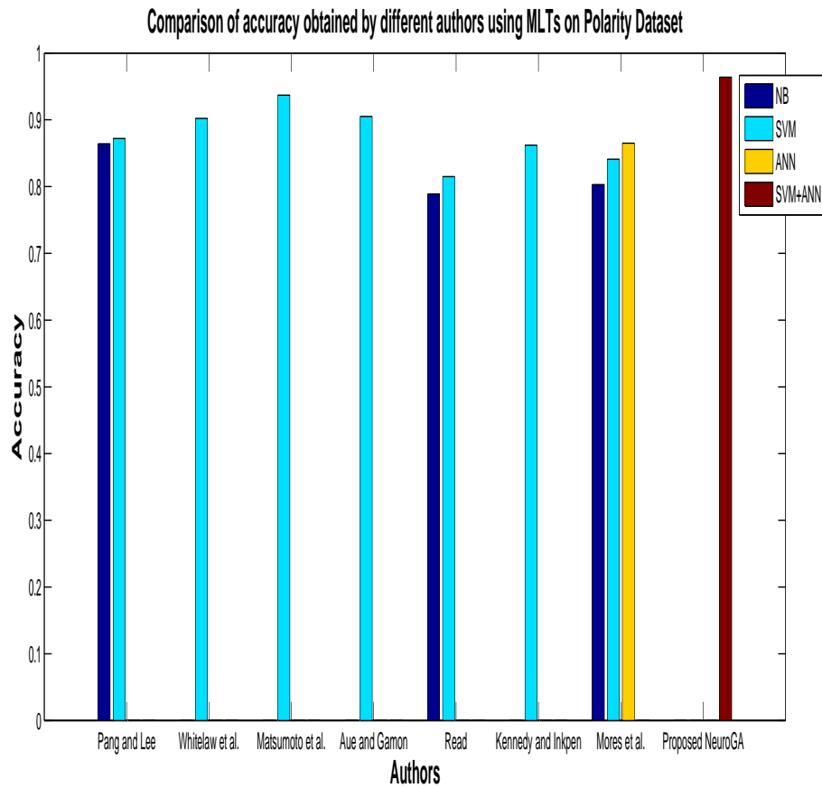
Figure 6.5: Comparison of accuracy values of obtained by different authors on Polarity dataset
