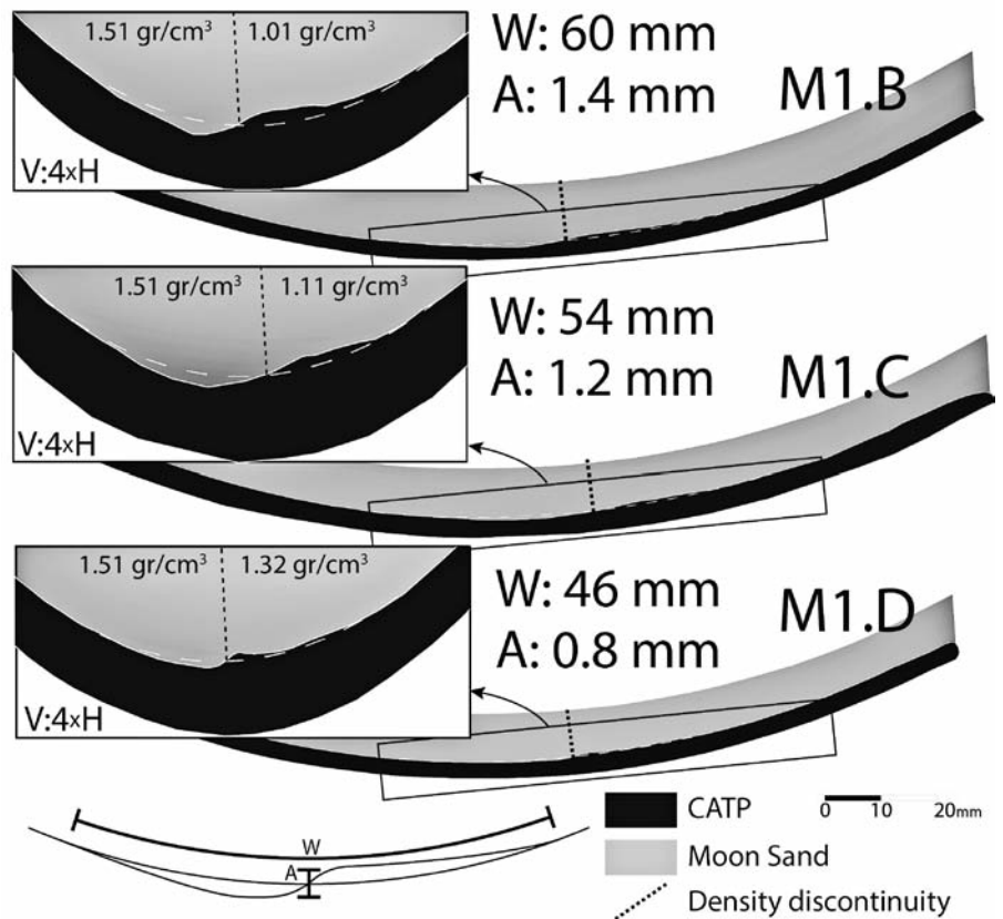
Fig. 1.- Interpreted sketches from cross-section at the end of experiments and detail of the structure that developed near the density discontinuity (vertically exaggerated). Dimensions of syncline-anticlines structures are characterized by their wavelength (W) and amplitude (A).
