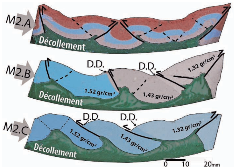
Fig. 2.- Interpreted cross-sections of compressional models. Density is indicated and density discontinuities (D.D.) displayed and labelled. See colour figure on the Web.
