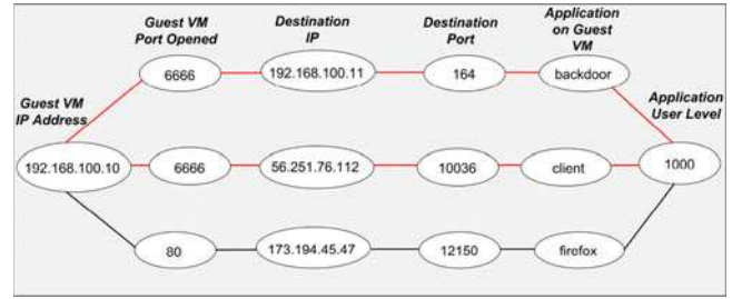
Fig. 3. Potential attack paths in the correlation graph as flagged up by MapReduce parser.
