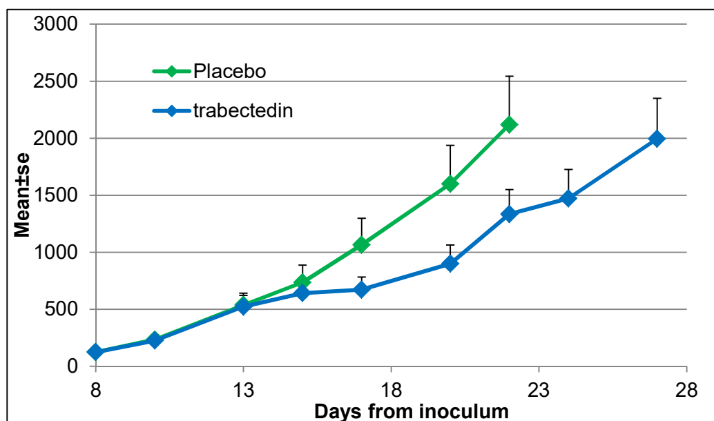
Figure 52: Antitumor activity of trabectedin (blue line) in TC71 xenograft model, compared to a placebo (green line).
