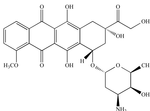
Figure 11: chemical structure of doxorubicin.
