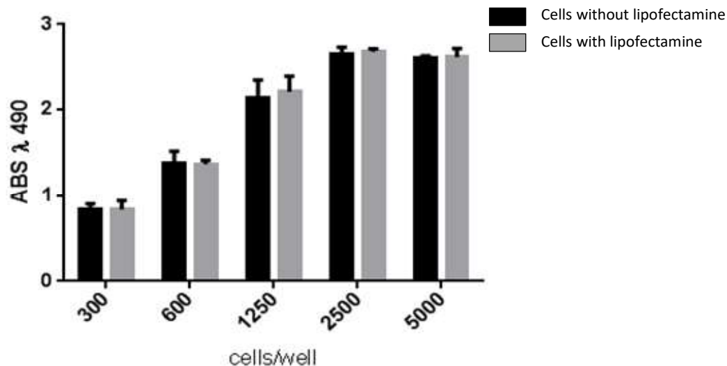
Figure 54 - Panel A: Evaluation of the toxicity of lipofectamine (0.05 \mu\text{l/well} ) in TC71 cells. The cells were seed at different concentrations in 384 wells/plate and treated with lipofectamine or with medium (as control), 48 hours later. The time 48 hours was selected by previous experiments performed to determine the point in which the cytotoxicity was visible and the phenomenon of confluence in the control cells (not treated) was not reached. The evaluation was performed by MTS assay, 48 hours after transfection. The values represent the mean of six replicates. Bars \pm sd.
