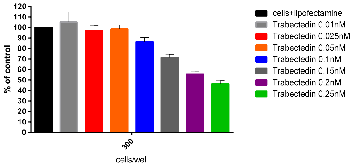
Figure 56: Evaluation of the toxicity induced by 48 hours of exposure to different concentrations of trabectedin. TC71 cells, seeded in 384 well/plates at the concentration of 300 cells/well, were treated 48 hours later, when reached the exponential phase. The evaluation was performed by MTS assay, 48 hours after treatment. The values represent the mean of six replicates. Bars \pm sd.
