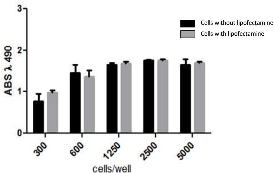
Figure 54 - Panel A: Evaluation of the toxicity of lipofectamine (0.05 \mu\text{l/well} ) in TC71 cells. The cells were seed at different concentrations in 384 wells/plate and treated with lipofectamine or with medium (as control), 48 hours later. The time 48 hours was selected by previous experiments performed to determine the point in which the cytotoxicity was visible and the phenomenon of confluence in the control cells (not treated) was not reached. The evaluation was performed by MTS assay, 48 hours after transfection. The values represent the mean of six replicates. Bars \pm sd.
