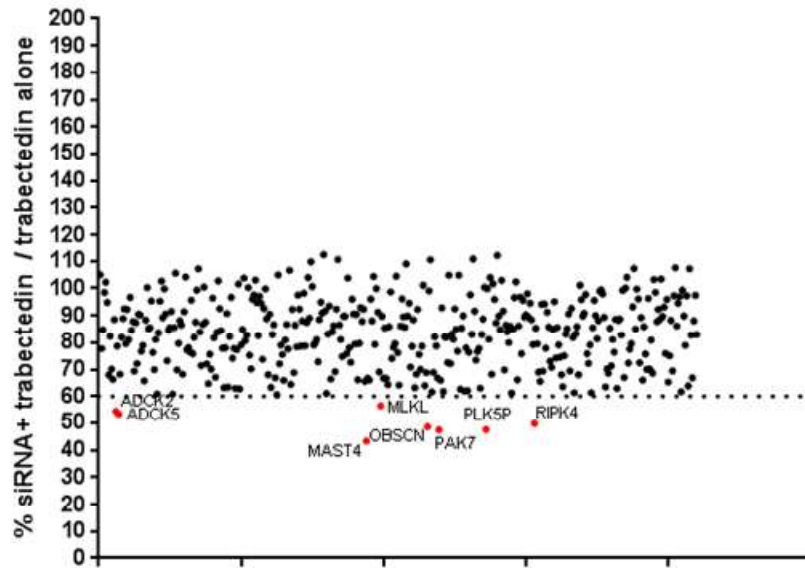
Figure 62: schematic representation of the results obtained by the transfection with the first part of the siRNA library using the analysis \text{siRNA} + \text{trabectedin} / \text{trabectedin alone} \times 100 .
