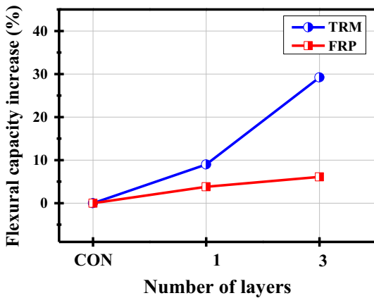
Fig. 12. Effect of the number of layers on the ultimate flexural capacity at 150 °C.
