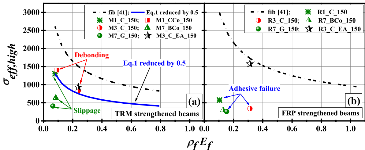
Fig. 13. Experimentally obtained effective stress versus \rho_f E_f and comparison with the theoretical formula suggested by fib 2010 [41] and its modification for 150 °C for (a) TRM and (b) FRP strengthened beams.
