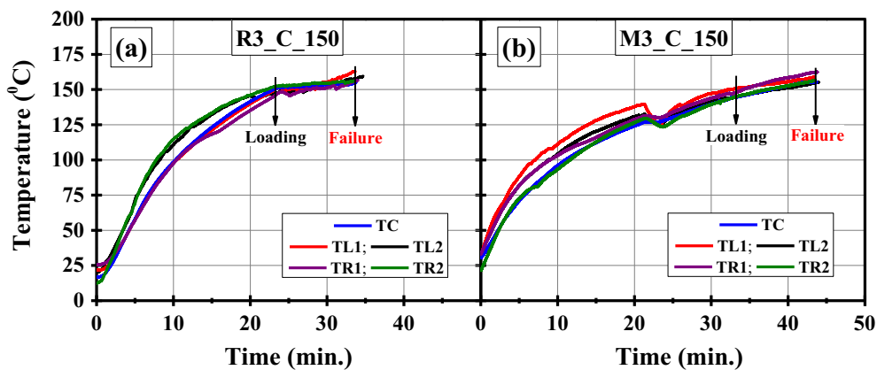
Fig. 6. Temperature-time curves: (a) FRP-strengthened beam (R3_C_150), and (b) TRM-retrofitted beam (M3_C_150).
