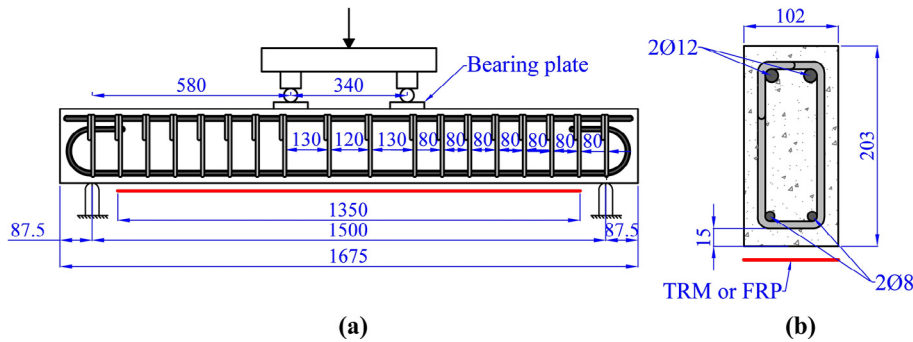
Fig. 1. Details of test beams: (a) Beam geometry and reinforcement; (b) cross section (dimensions in mm).
