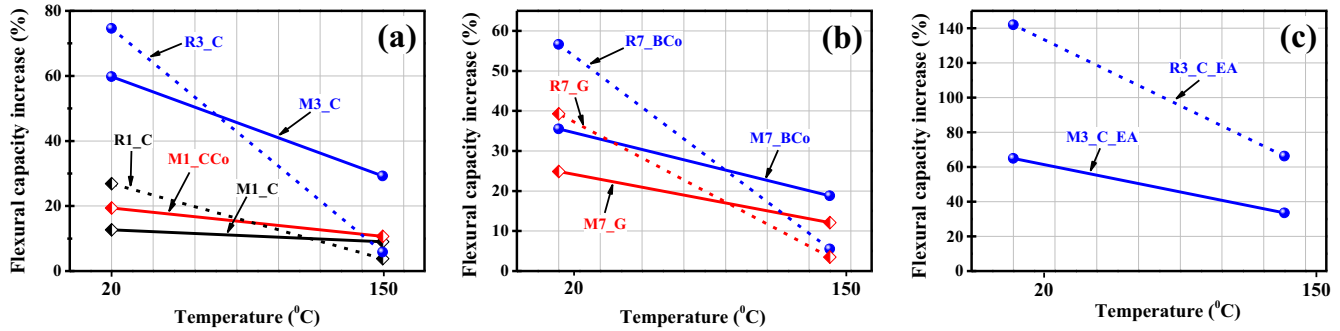
Fig. 10. Effect of temperature on the flexural capacity enhancement for both TRM and FRP system.
