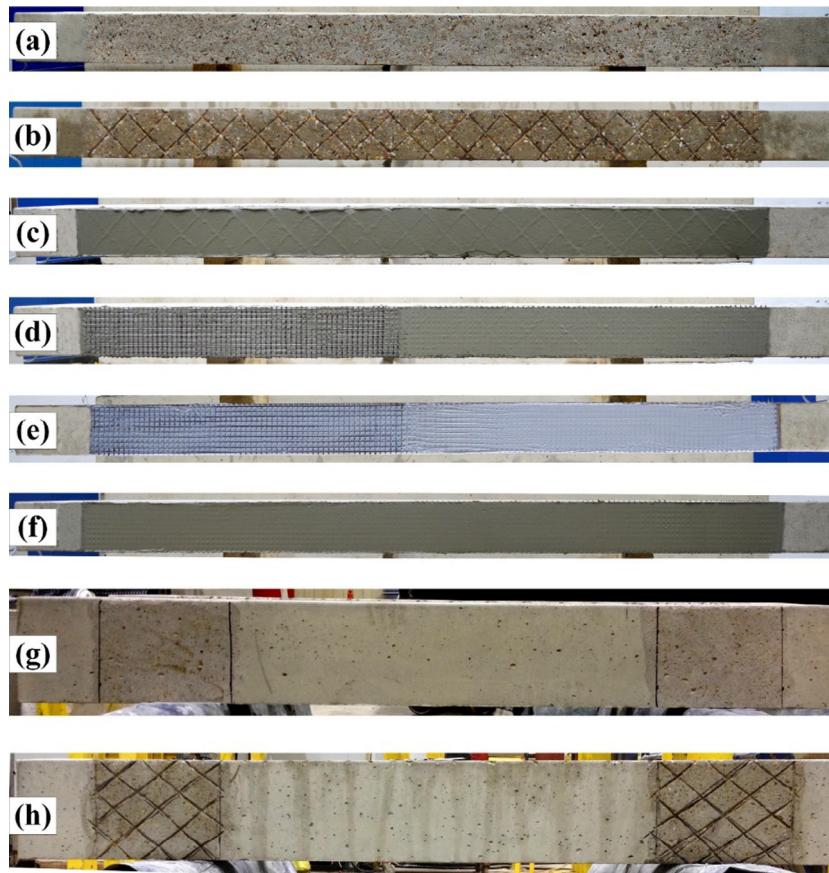
Fig. 4. Strengthening procedure: (a) surface preparation of FRP-strengthened beams, (b) surface preparation of TRM-retrofitted beams, (c) application of first layer of mortar, (d) application of first layer of TRM, (e) application of the first layer of FRP, (f) application of final layer of mortar for TRM reinforced specimens, (g) surface preparation of FRP U-shaped jacket, (h) surface preparation for TRM U-shaped jacket.
