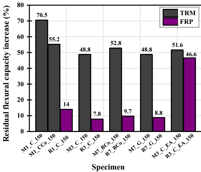
Fig. 11. Comparison of residual flexural capacity increase of TRM vs. FRP strengthened beams at 150 °C.
