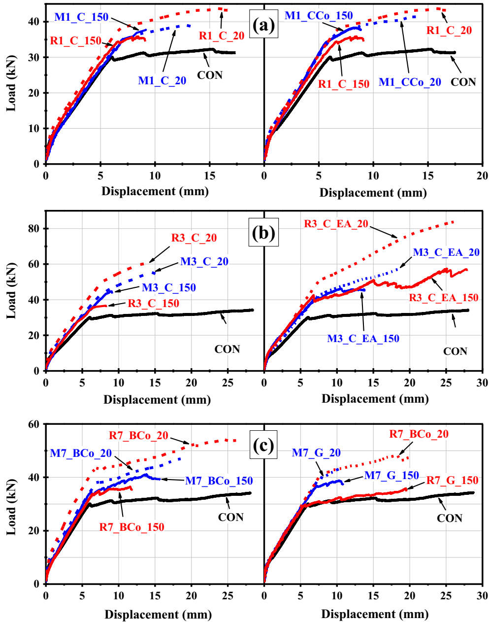
Fig. 7. Load versus mid-span deflection curves of beams tested at ambient and high temperature and strengthened with: (a) one layer of carbon fibres textile, (b) three layers of carbon fibres textile without and with providing end-anchorage system, and (c) seven layers of basalt or glass fibres textile.
