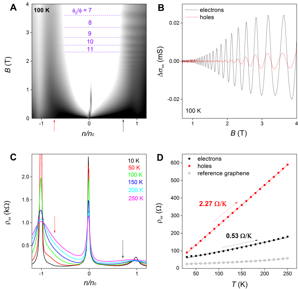
Figure S7 | Electron-hole asymmetry of Brown-Zak oscillations. a , \sigma_{xx} as a function of n and B , similar to Fig. 2B but for a superlattice device with a \approx 13.6\text{ nm} . The grey scale is logarithmic: white 0.09\text{ mS} ; black 5\text{ mS} . b , After subtracting a smooth background, \Delta\sigma_{xx}(B) is plotted for the fixed n \approx \pm 1.7 \times 10^{12}\text{ cm}^{-2} [ n/n_0 \approx \pm 0.7 ]. These electron and hole concentrations are marked by the black and red arrows in (a), respectively. c , \rho_{xx} for the same device as a function of n at various T in zero B (the curves are color coded). The resistivity increases with T faster for holes than electrons and much faster than in reference devices. d , Detailed T -dependence for electrons and holes at the same n as in (b). Dots – experiment;
