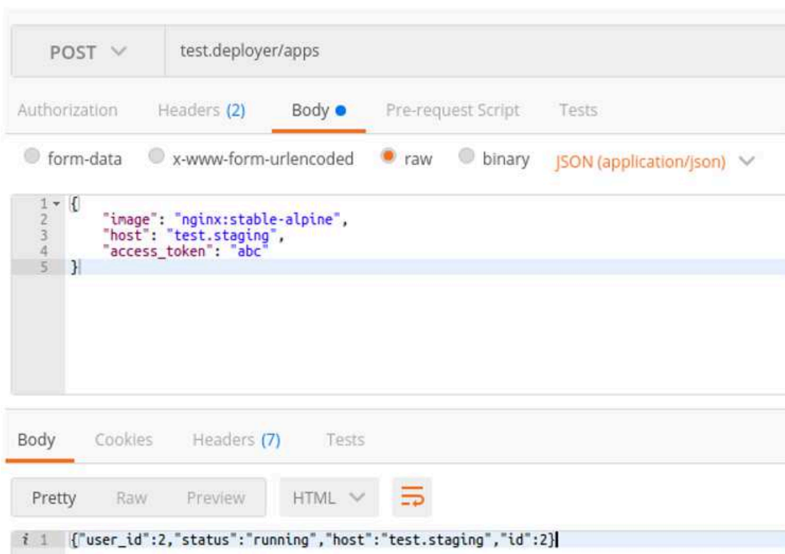
Figura 20 – Postman executando o endpoint POST/apps
