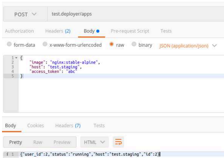
Figura 12. Postman executando o endpoint POST/apps
