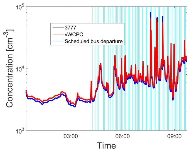
Figure 10. Concentration measured by the 3777 and vWCPC from urban atmospheric air.
