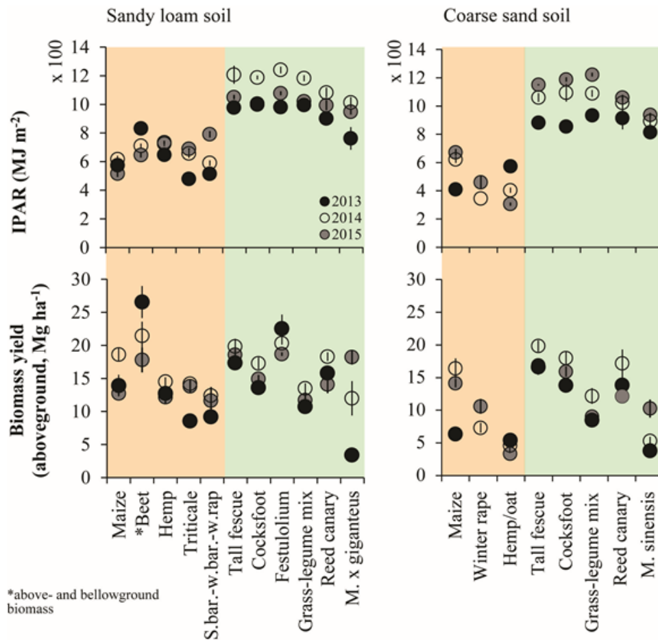
Figure 3. Interception of photosynthetically active radiation (IPAR) in annual (orange shade) and perennial (green shade) crops during 2013-2015 on two soil types at AU (from Manevski et al., 2016).
