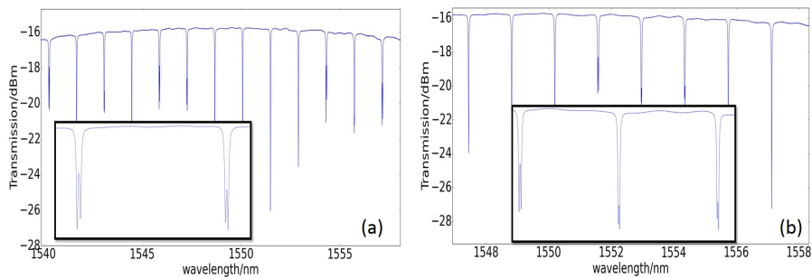
Fig. 6. Two measured spectra of simple ring resonators (without reflectors) on the same chip, located close to the ring resonator with tunable reflector. Both rings, which have different coupling conditions, show clear resonance-splitting in most resonance peaks.
