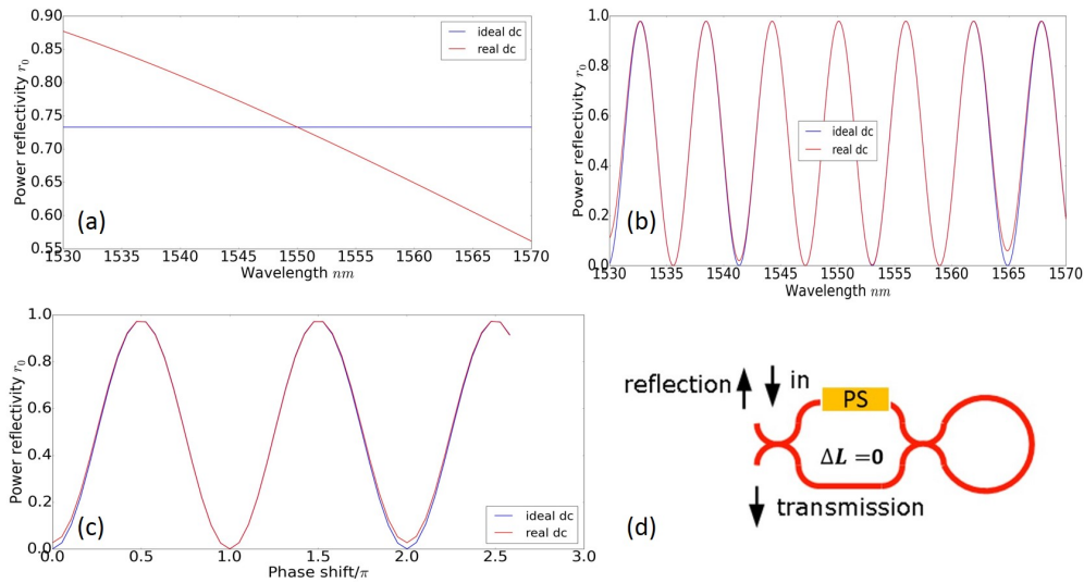
Fig. 3. Simulated reflection spectrum of the tunable reflector. (a) \Delta L = 0 produces a flat spectrum. (b) \Delta L = 50 shows a strong, periodic wavelength dependence oscillating between 0 and 100%. (c) Adding 0.5\pi phase shift in one arm can generate a change in reflectivity from 0 to 100%. Blue and red corresponds with an ideal directional coupler case and a realistic directional coupler case, respectively. The reflection does not reach 100% because of the small propagation loss of the waveguides which is taken into account. (d) shows the reflector with a phase shifter used to simulate the tunability.
