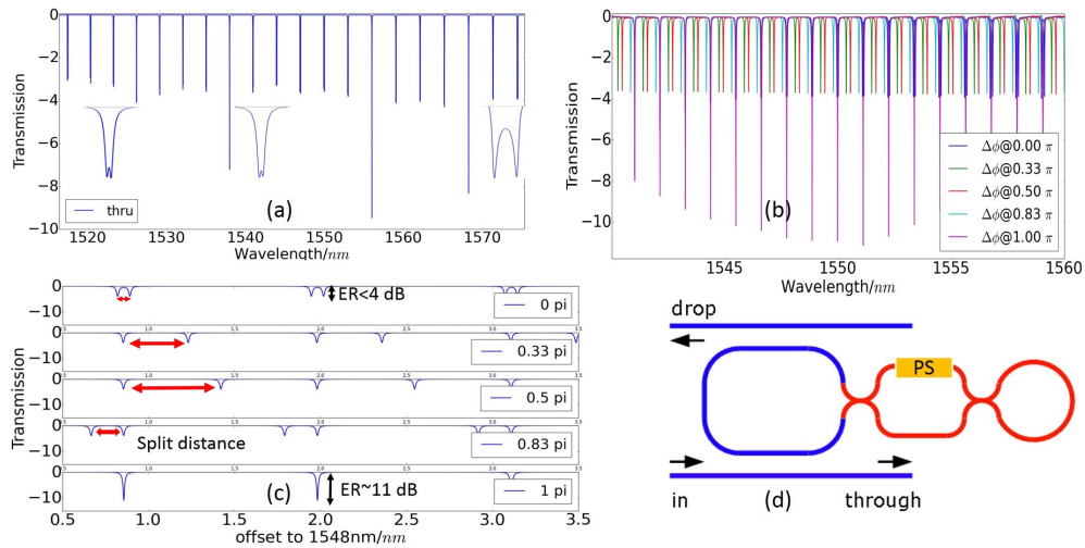
Fig. 4. Simulated through port spectrum of a ring circuit with only backscattering and other parasitics in the circuit, including reflections and backcoupling at the directional couplers (a), and with both backscattering and tunable reflector (b) and (c). It shows clearly how the resonance shape evolves with phase shift. (d) gives the brief schematic of the device with a phase shifter.
