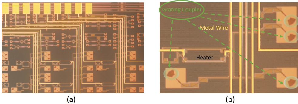
Fig. 5. (a) gives the overall view of the devices fabricated after heater processing, (b) presents a zoomed view of one specific device.
