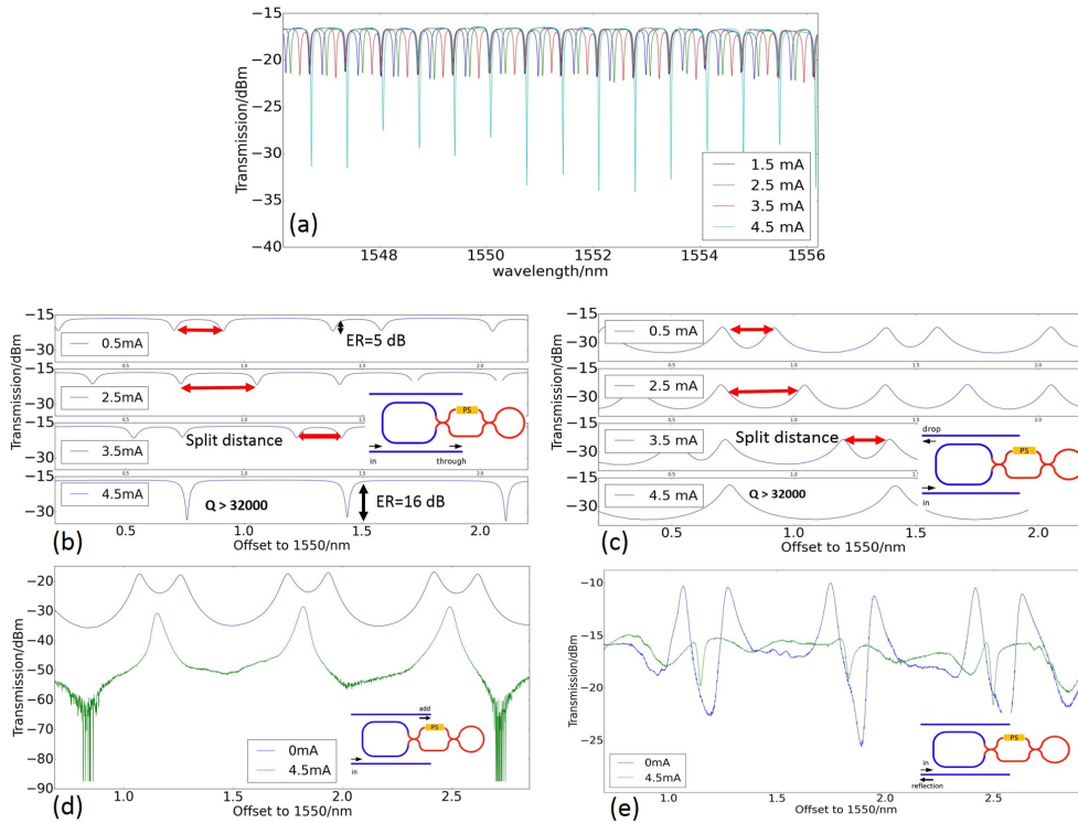
Fig. 7. Experimental measurements of compensated backscattering. (a) demonstrates the control of all the resonances. (b) gives a zoomed-in view about how the resonance shapes evolve from clearly split to non-split. (c) shows the same compensation for the output at the drop port, while (d) and (e) show how our device can suppress the unwanted output from add and in port.
