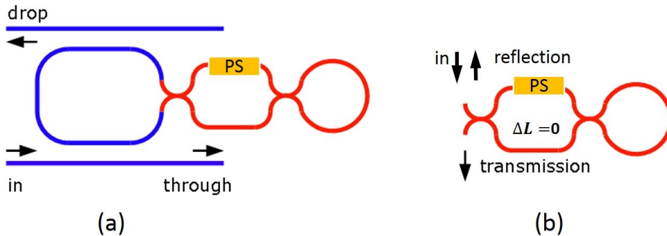
Fig. 2. Schematics of the ring with a reflector and the reflector itself, respectively.
