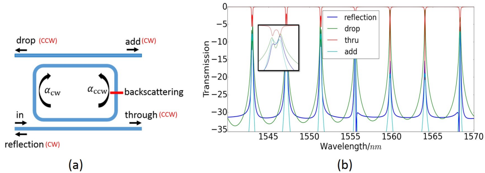
Fig. 1. (a) shows a brief schematic for a ring resonator with backscattering, which is modelled by a lumped reflector. (b) gives the simulated spectra of such a ring resonator to demonstrate the effects of backscattering in the circuit. Note the clear resonance splitting in through and drop port, and the high transmission in add port and in port.
