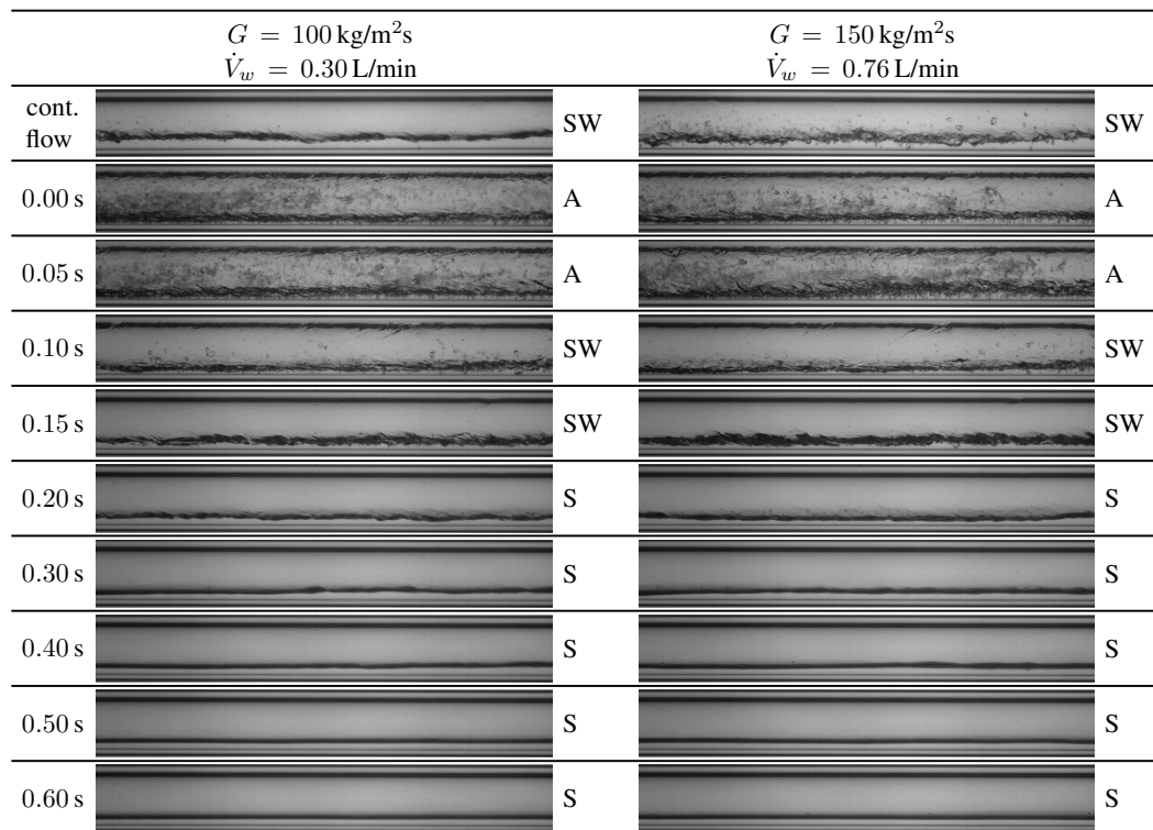
Figure 12: Visualization of continuous and pulsating flow (valve closing) immediately after the EXVs
