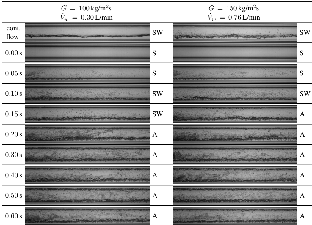
Figure 11: Visualization of continuous and pulsating flow (valve opening) immediately after the EXVs
