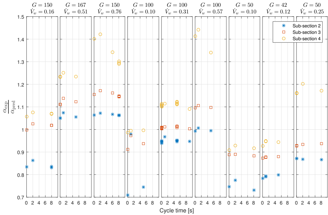
Figure 8: Normalized heat transfer coefficients calculated by the Fang (2013) correlation vs. cycle time at various refrigerant mass fluxes and water volume flows. Continuous flow results are located at 0 cycle time.
