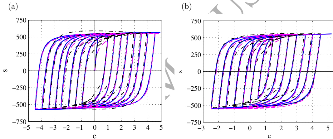
Figure 4: Symmetric cycling: Shi et al. (2012) experiment (—), model (---). Present model (--).
