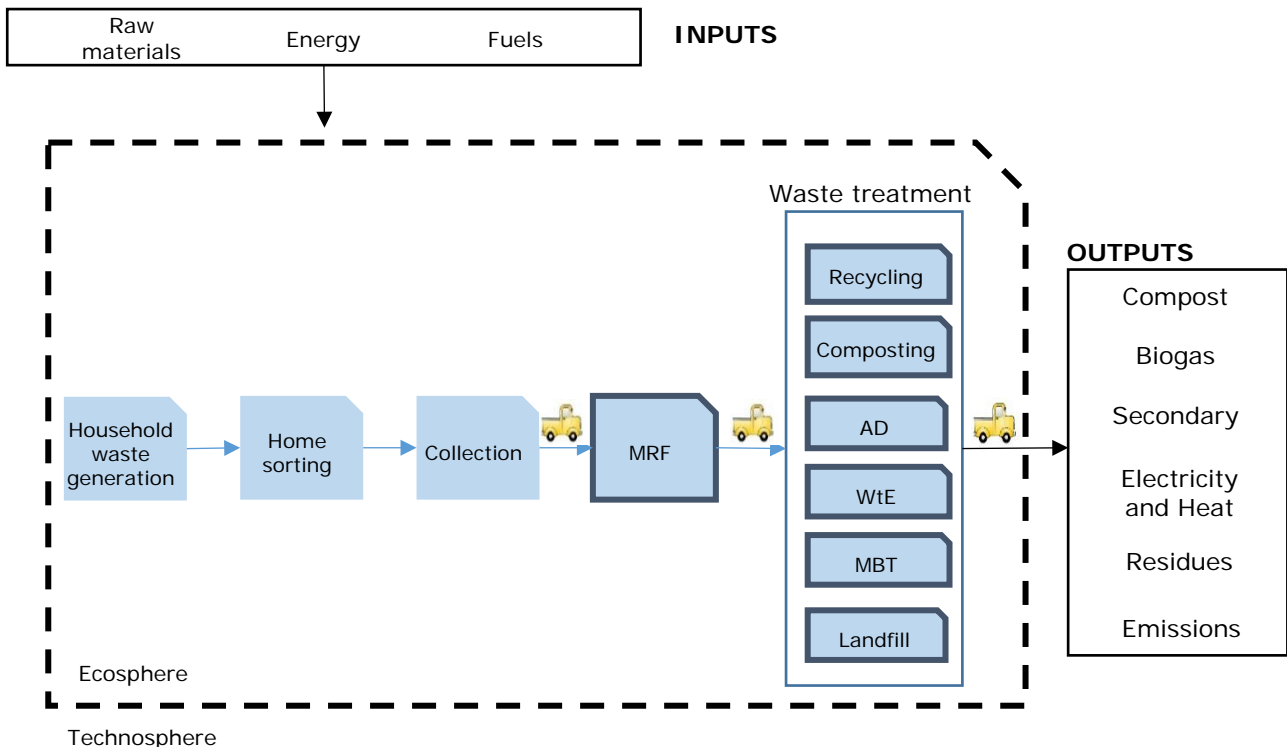
Figure 1: System boundaries of the LCA study. The truck indicates the inclusion of the waste transportation. The thicker border indicates the inclusion of capital goods in the process
