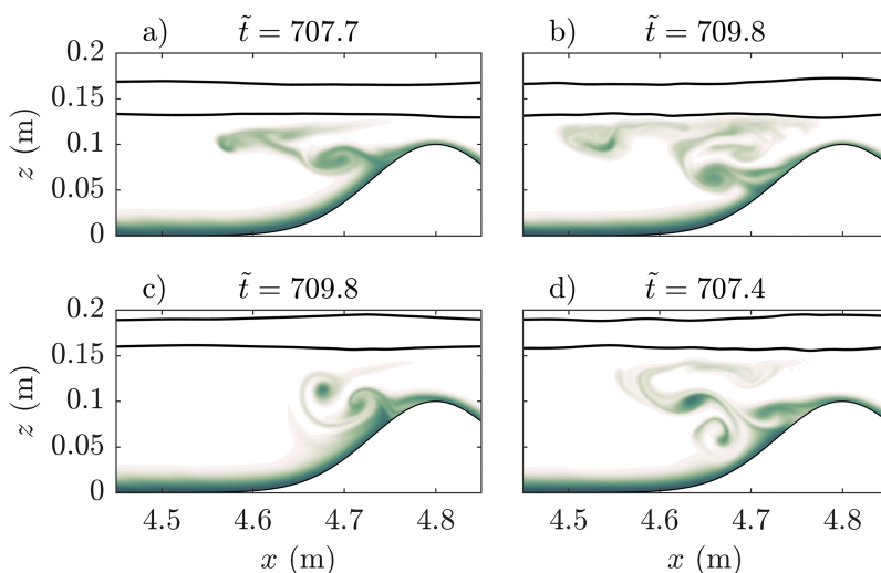
FIG. 11. Passive tracer well after the transit of the mode-2 ISW for numerical cases (a) 3008, (b) 3010, (c) 3510, and (d) 3512. Moderate (strong) interaction corresponds to the left (right) column. The colour scale is the same as Fig. 10.
