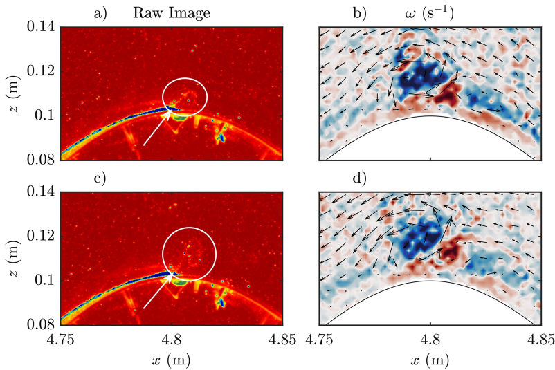
FIG. 4. False colour of the raw image [(a) and (c)] and vorticity [(b) and (d)] for moderate vorticity roll-up (experimental case 040516). [(a) and (b)] 34.7 non-dimensional time units (6.7 s) after the wave crossed directly over the hill peak and [(c) and (d)] 6.5 non-dimensional time units (1.25 s) later. In the left column, the circle emphasizes the resuspended particles and the arrow points to the separation point. The vorticity colour scale is the same as the right column of Fig. 3.
