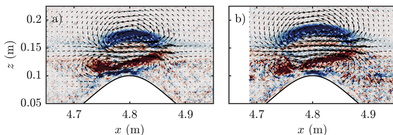
FIG. 8. Vorticity and velocity vector field for [(a), (c), and (e)] globular extraction (experimental case 060516) and [(b), (d), and (f)] filamentary extraction (experimental case 290416) at the moment the wave is directly above the hill crest. The colour scale is the same as the right column of Fig. 3.
