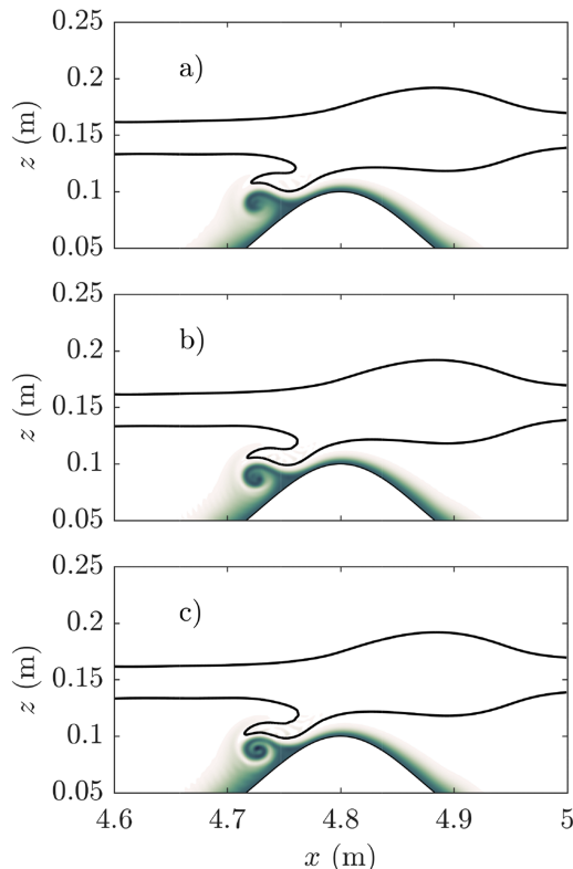
FIG. 12. Passive tracer for strong interaction (numerical case 3010) at \bar{t} = 473.2 with (a) Re = 129 , (b) Re = 257 , and (c) Re = 514 . The colour scale is the same as Fig. 10.
