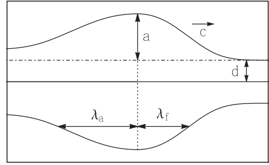
FIG. 2. Schematic of parameters for a rightward moving mode-2 ISW. Adapted with permission from “Mass transport by mode-2 internal solitary-like waves,” Phys. Fluids 28 , 056606 (2016). Copyright 2016 AIP Publishing LLC.
