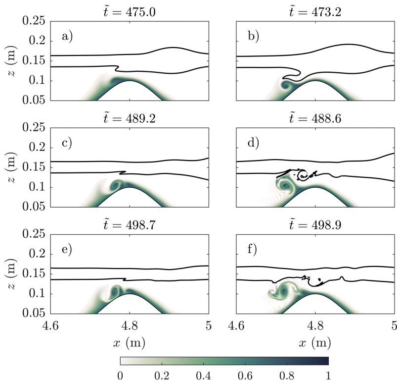
FIG. 10. Passive tracer for [(a), (c), and (e)] moderate (numerical case 3008) and [(b), (d), and (f)] strong (numerical case 3010) interactions.
