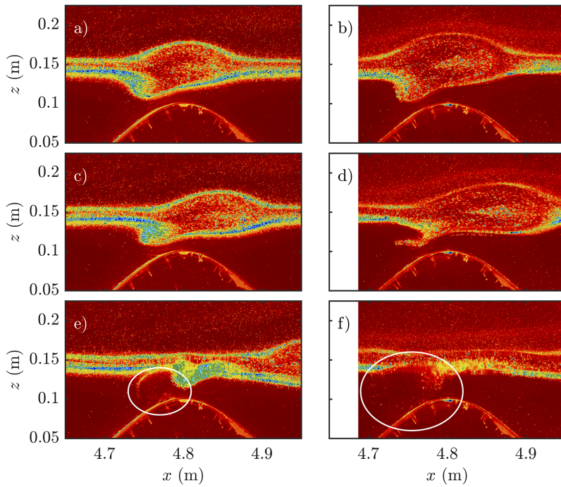
FIG. 7. False colour time series of the raw image for the mass extraction of type: [(a), (c), and (e)] globular extraction (experimental case 060516) and [(b), (d), and (f)] filamentary extraction (experimental case 290416). (c) and (d), and (e) and (f) are 6 and 23 non-dimensional time units after (a) and (b), respectively.
