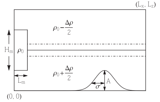
FIG. 1. Initial tank configuration (side view). Horizontal lines denote the location of the pycnocline centre (solid line) and pycnocline half-width (dashed-dotted lines). The intermediate region with height H_m and width L_m contains density \rho_0 and is centred on the pycnocline (left end of the tank). Figure not to scale.
