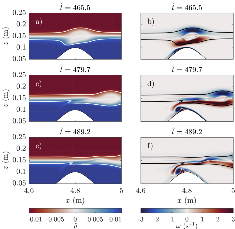
FIG. 3. Density anomaly [(a), (c), and (e)] and vorticity [(b), (d), and (f)] for a moderate interaction (numerical case 3008). White (black) contours in the left (right) column are the characteristic isopycnals.
