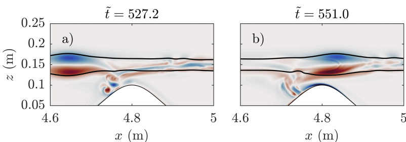
FIG. 5. Vorticity of the second mode-2 ISW for moderate interactions (numerical case 3008). The colour scale is the same as the right column of Fig. 3.
