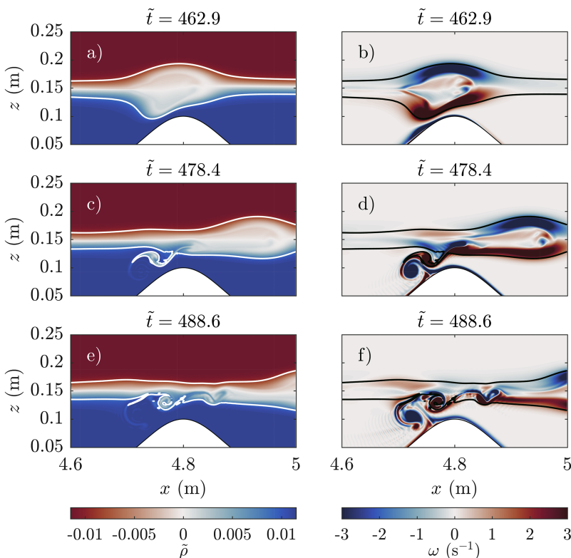
FIG. 6. Density anomaly [(a), (c), and (e)] and vorticity [(b), (d), and (f)] for the strong interaction (numerical case 3010). All other contours are the same as in Fig. 3.
