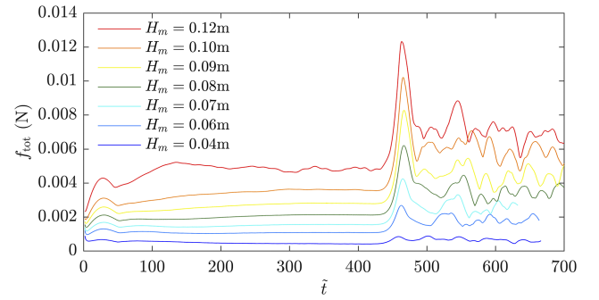
FIG. 9. Variation of total bottom surface stress, f_{\text{tot}} , with non-dimensional time, \tilde{t} , for fluid depth L_z = 0.30 \text{ m} and H_m values shown (numerical cases 3004–3012).
