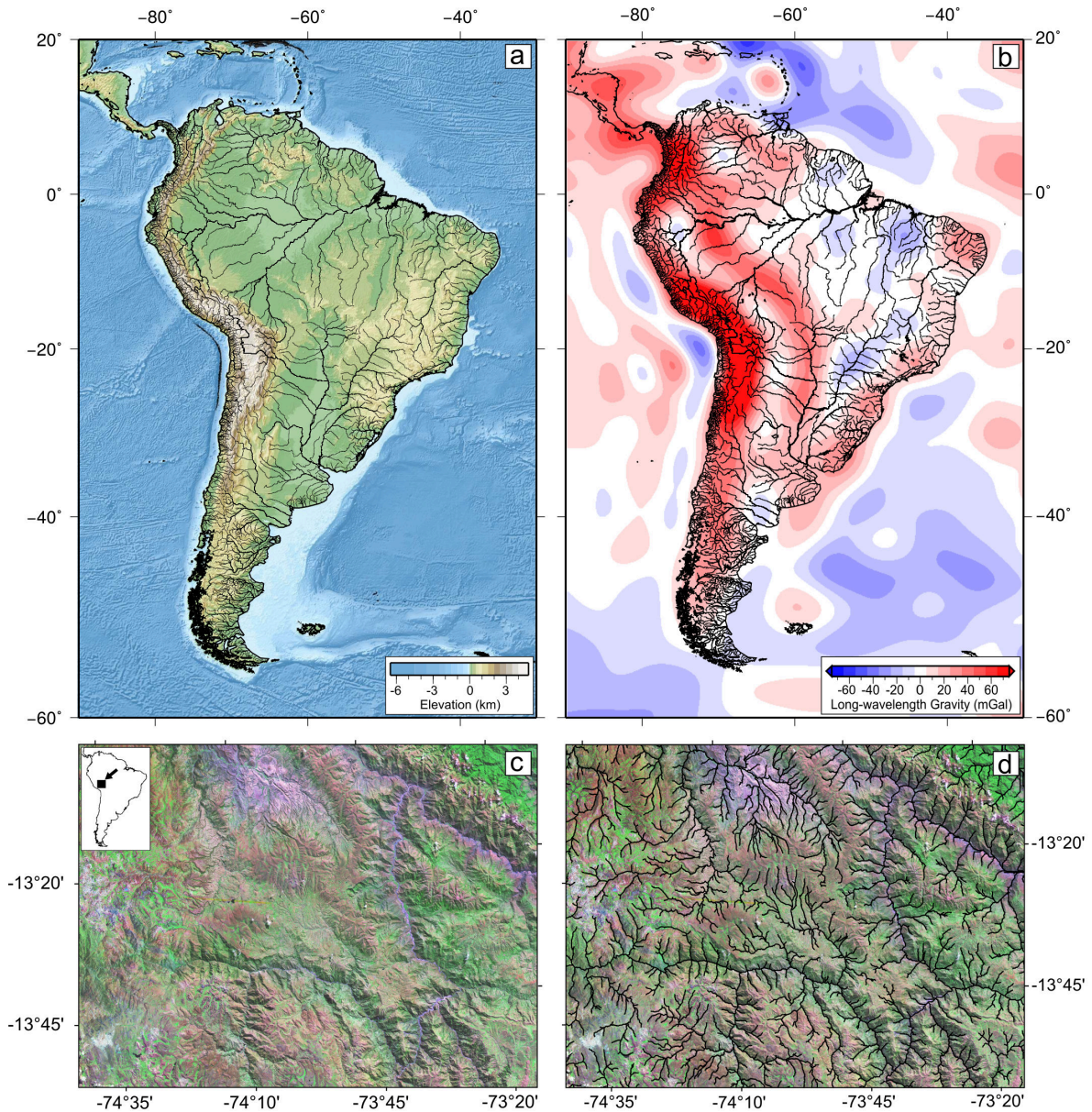
Fig. 3: (a) Topographic map of South America overlain with drainage network comprising 1827 rivers extracted from Shuttle Radar Topography Mission (SRTM) dataset. (b) Long wavelength ( > 730 km) non-hydrostatic free-air gravity anomaly map overlain with drainage network (Mayer-Guerr, 2015). (c) Landsat satellite image from Central Peruvian Andes showing drainage network. Inset shows location. (d) Same image as (c) overlain with recovered drainage network.
