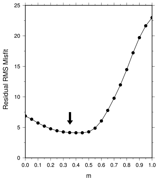
Fig. 7: Residual RMS misfit between observed and calculated river profiles plotted as function of m . Arrow = optimal value of m = 0.35 . Note shallow global minimum at m = 0.3 – 0.5 .
