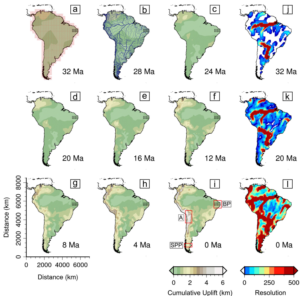
Fig. 6: Calculated cumulative uplift history of South America (i.e. \int_0^t U(x, y, t) dt ) as function of space and time. (a) Cumulative uplift at 32 Ma. Red circles = spatial distribution of grid points at which uplift rate can vary during inversion; Black dots = nodes from Borborema Province where erosional parameters were calibrated. (b) Cumulative uplift at 28 Ma. Blue lines = 1827 river profiles used for inverse modeling. (c)–(i) Snapshots of cumulative uplift from 24 Ma to present day. BP = Borborema Province; A = Central Andean Altiplano; SPP = Southern Patagonian Plateau. (j)–(l) Selected panels at three different times showing number of non-zero entries in model matrix, M , for given uplift nodes.
