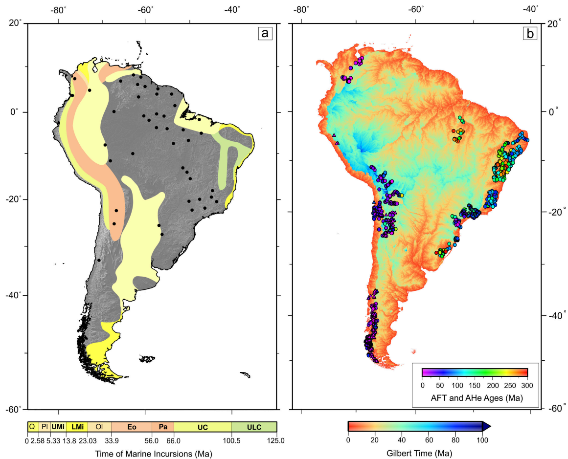
Fig. 4: (a) Schematic Cenozoic and Mesozoic paleogeographic map of South America. Colored polygons = age and extent of post-Mesozoic marine incursions from distribution of marine and coastal strata (after Lundberg et al. , 1998; Arai, 2014); black circles = bauxite/laterite deposits (after Lima da Costa, 1993). (b) Landscape response time, \tau_G , calculated from digital elevation model using Equation (3) with m = 0.35 and v = 10 . Colored circles/triangles = AFT and A-He ages (Restrepo-Moreno et al. (2009); Parra et al. (2009); Bermúdez et al. (2010, 2011); Villagómez et al. (2011); Michalak et al. (2016) for the Northern Andes; selected references from compilation in Barnes & Ehlers (2009) for Central Andes; Thomson et al. (2001, 2010); Haschke et al. (2006); Guillaume et al. (2013) for Southern Patagonian Andes; Gallagher et al. (1994); Harman et al. (1998); Hackspacher & Ribeiro (2004); Turner et al. (2008); Morais Neto et al. (2009); Franco-Magalhaes et al. (2010, 2014); Hiruma et al. (2010); Cogné et al. (2011, 2012); Japsen et al. (2012); Jelinek et al. (2014); Oliveira et al. (2016) for South American Platform).
