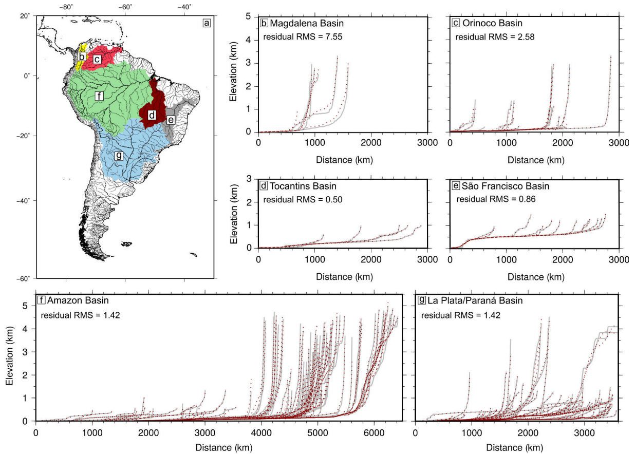
Fig. 5: Inverse modeling of 1827 South American river profiles. (a) Drainage map. Colored polygons = 6 largest catchments, where labels correspond to panels (b)–(g). (b)–(g) Gray/red lines = observed and calculated river profiles, respectively. In each case, residual RMS misfit for the catchment is given.
