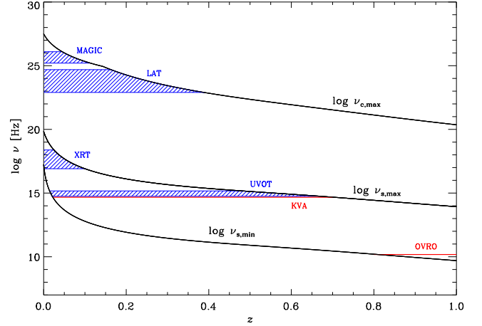
Figure 4. The trend of the observed frequencies as a function of the distance along the helical jet axis z (whose unit length can be estimated to be about 0.1 pc, see the text). The location of the regions that contribute to the emission observed by the various instruments is highlighted. The plot refers to the high-emission state shown in Fig. 5.
