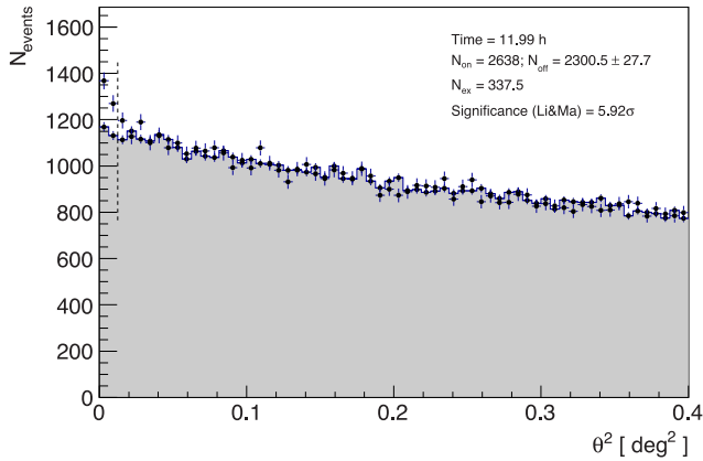
Figure 1. \theta^2 distribution of signal (black points) and background (grey area) events. N_{\text{on}} is the number of all events with \theta^2 < 0.0125 \text{ deg}^2 (vertical dashed line) with respect to the source position in the camera, and N_{\text{off}} the normalized number of all events from the same region around OFF-source position.
