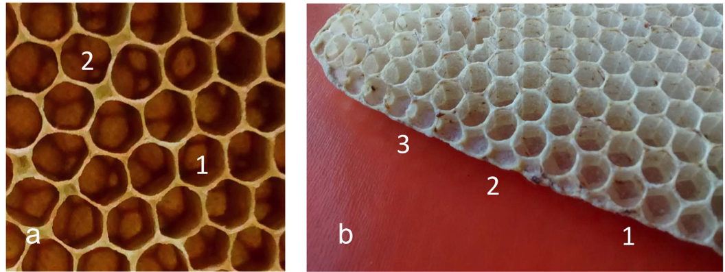
Figure 1. Geometry and construction of the honeycomb. (a) The pattern of cells influences their final shape: cell 1, surrounded by six other cells, has a hexagonal shape, with 120^\circ angles between sides, whereas cell 2 has a different shape, with 90^\circ angles between some consecutive sides. (b) The margin of a comb with stubs of cells at different stages of construction suggests a possible construction scheme (1: the construction of the cell base is started in the groove between two pre-existing cells; 2: when the cell base is as large as the cell diameter, the walls are started; 3: the walls encircle the first stub of the cell).
