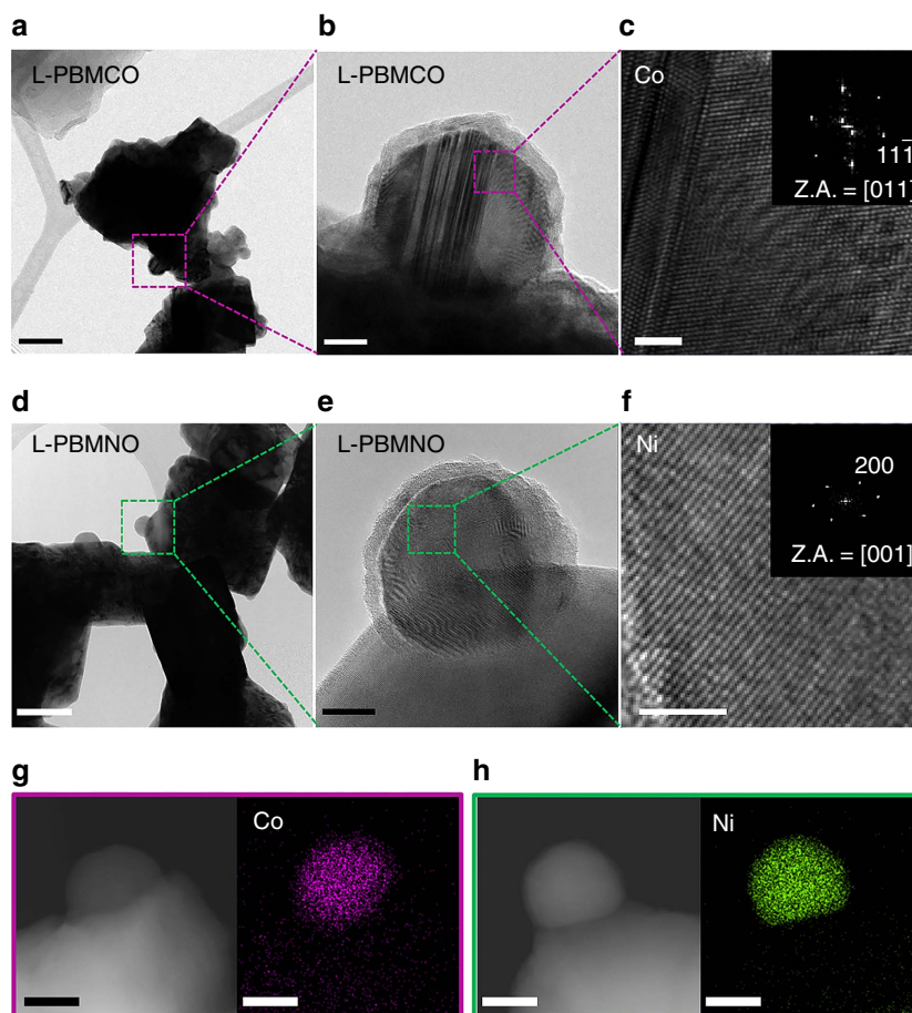
Figure 1 | Transmission electron microscopic analysis. (a) A bright-field (BF) TEM image; scale bar, 100 nm and (b) high-resolution (HR) TEM image of \text{PrBaMn}_{1.7}\text{Co}_{0.3}\text{O}_{5+\delta} (L-PBMCO) sample; scale bar 10 nm. (c) Magnified HR TEM image of exsolved Co nanoparticle; scale bar 2 nm, (d) BF TEM image; scale bar 100 nm and (e) HR TEM image of \text{PrBaMn}_{1.7}\text{Ni}_{0.3}\text{O}_{5+\delta} (L-PBMNO) sample; scale bar 10 nm. (f) Magnified HR TEM image of Ni nanoparticle; scale bar 2 nm. (g) High-angle annular dark-field (HAADF) image of the L-PBMCO with the EDS elemental map of Co; scale bar 25 nm. (h) HAADF image of the L-PBMNO with the EDS elemental map of Ni; scale bar 25 nm.
