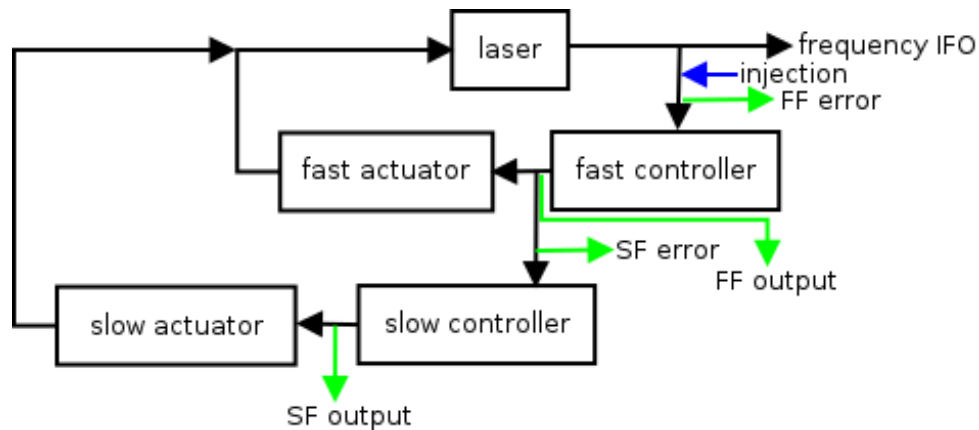
Figure 1. A simplified diagram of the laser frequency control loop. The quantities with the green arrows are housekeeping data channels and the frequency interferometer is a science data channel. The injected signal (blue arrow) cannot be downloaded.
