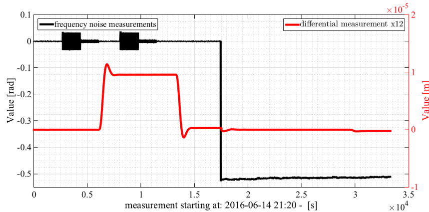
Figure 2. The concept of the arm length mismatch experiment. The black trace (corresponding to the left y -axis) shows the laser frequency noise measurement. The two sets of two injections are clearly discernible. The DC value of the signal is at a lower level during the open-loop measurement. The distance between the two test masses is shown in red (refer to right y -axis). The second set of modulations is taking place at the offset position. Some transients are discernible.
