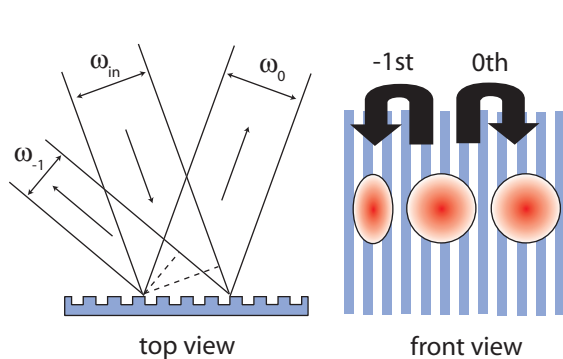
Figure 4. An all-reflective beam splitter always causes the beam profiles of the diffracted beams to be different with respect to each other. This is due to different deflection angles in the diffraction plane for the 0th and -1st diffraction order.
