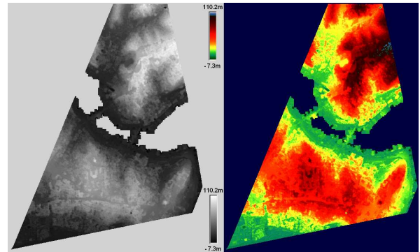
Figure 6. IKONOS DSM, grey value and color coded
