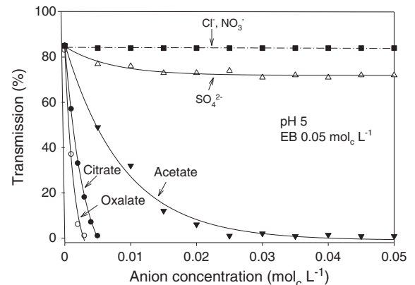
Fig. 3. Coagulation of the clay fraction in dependence on anion concentration.
