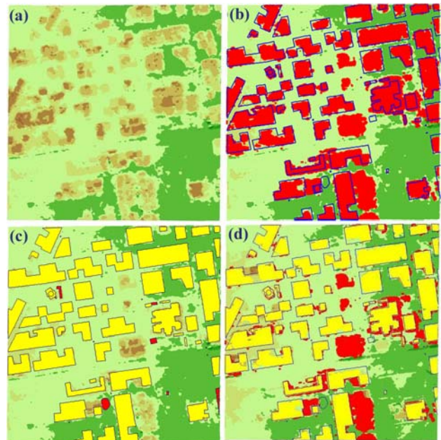
Figure 8. (a) IKONOS DSM of the whole scene, (b) IKONOS DSM superimposed with height blobs from nDSM in red, (c) GIS objects covered (yellow) and not covered (red) by height blobs, the latter being candidates for demolished buildings, (d) blobs (red) not covered by GIS objects, being candidates for new buildings.
