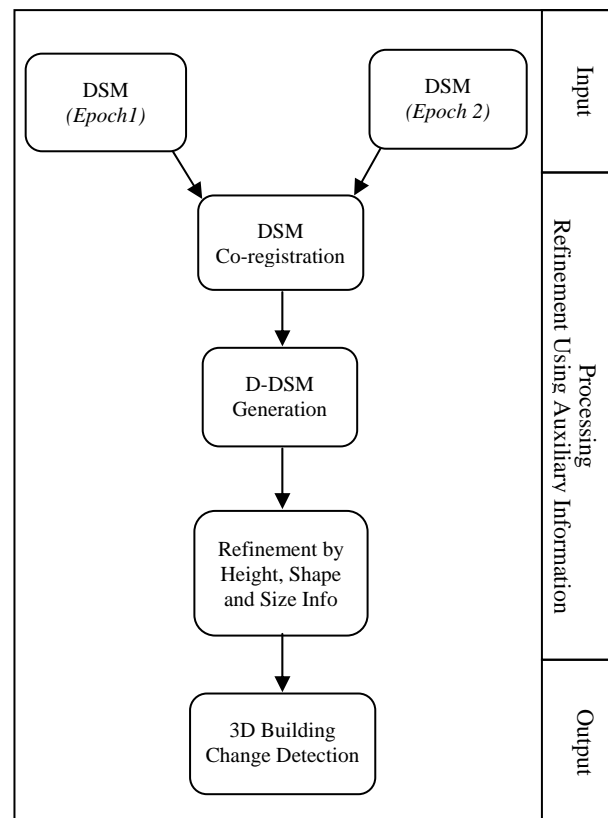
Figure 4. Diagram of 3D building change detection
