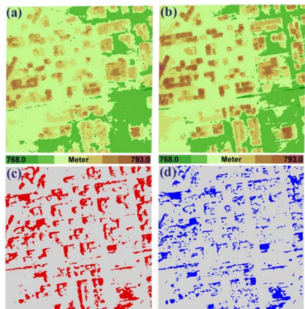
Figure 2. (a) IKONOS DSM, (b) GeoEye DSM, (c) and (d) binary change maps with D-DSMs larger than 2.5m: (c) before (red), and (d) after (blue) shift elimination
