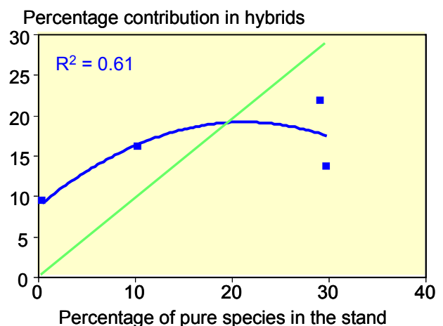
Figure 2-10. The pooled percentage of hybrids with the four species plotted against the percentage of the pure species in the Briouant stand in south-western France. The ideal relationship if the pure species would contribute to hybrids according to their occurrence in the stand is shown with the green line. Lepais et al. 2009.
