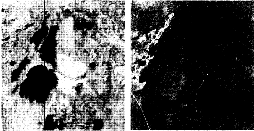
Figure 11. Band 94 (left) showing class 1 abnormal pixels and band 11 (right) showing class 2 abnormal pixels.
