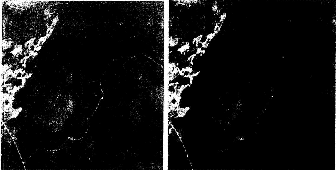
↑ ↑ ↑ ↑ ↑ ↑ ↑ Figure 44. Band 11 level 1a (left) and level 1b (right) Hyperion imagery, showing Class 2 abnormal pixel correction.
