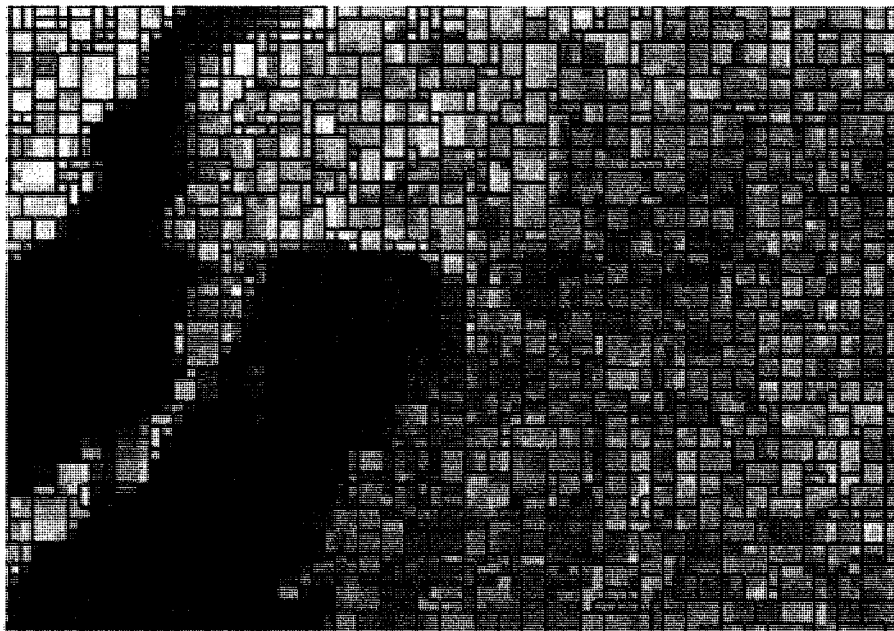
Figure 19. Level 2 segmentation.
