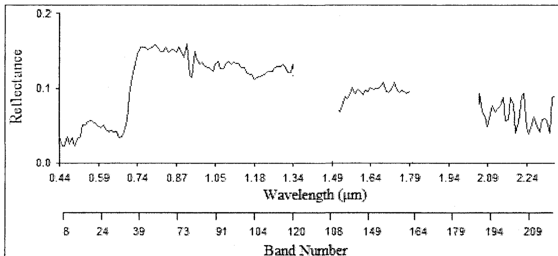
Figure 3. Spectral graph of jack pine, extracted from a Hyperion hyperspectral image.
