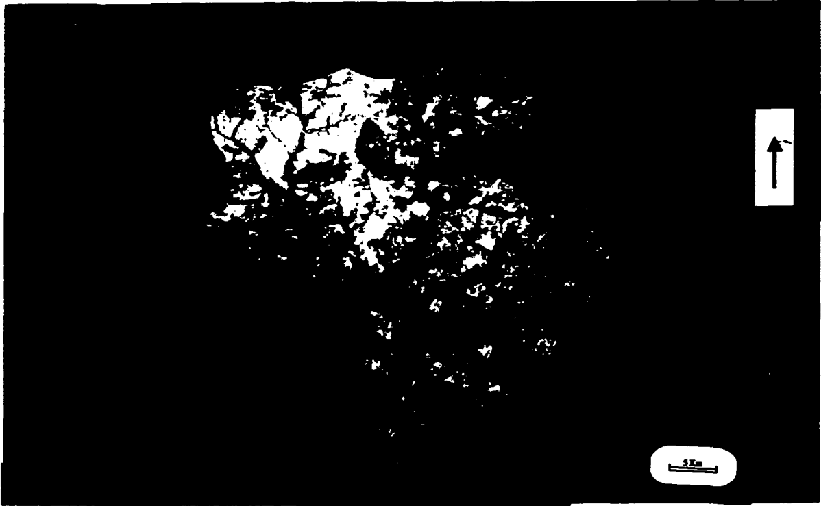
Figure 7. Landsat Multispectral Scanner (MSS) of Tamne River Basin, taken in 1975.
